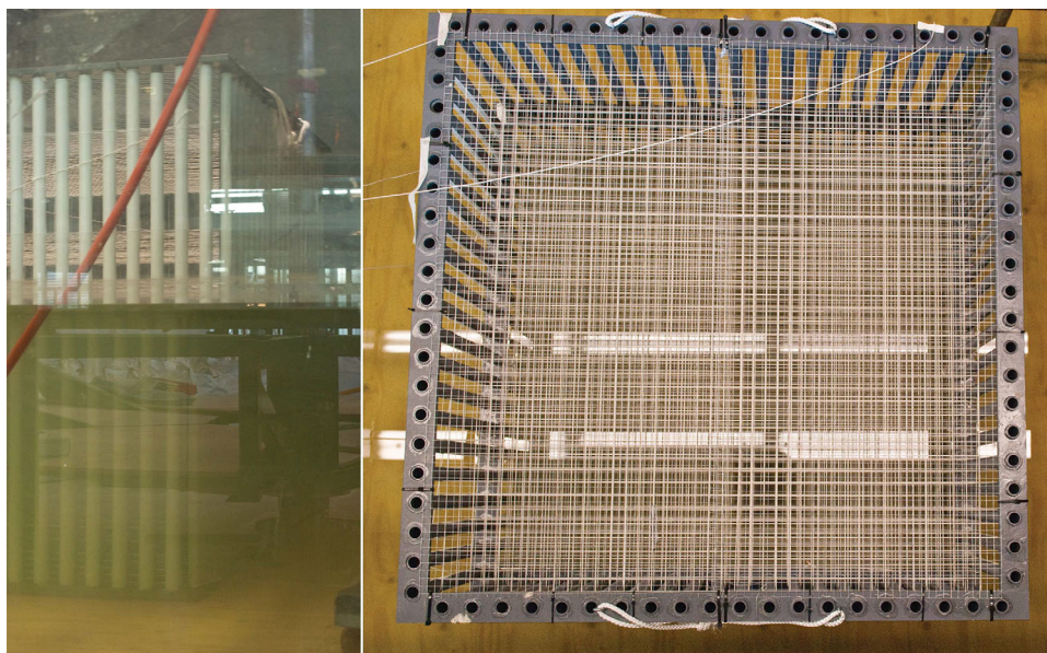
Figure 3. DTS setup deployed in a laboratory test setup.
