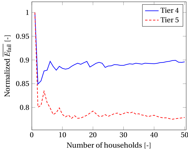
Figure 6.13: Variations in normalized average E_{fail} per household for homogeneous microgrids composed of tiers 4 and 5.
