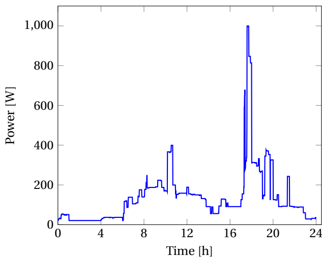
Figure 3.9: Load profile of an off-grid household with tier 4 electricity access for a representative day. Total energy consumption for this day is 3.29 kWh with a peak of around 1 kW.
