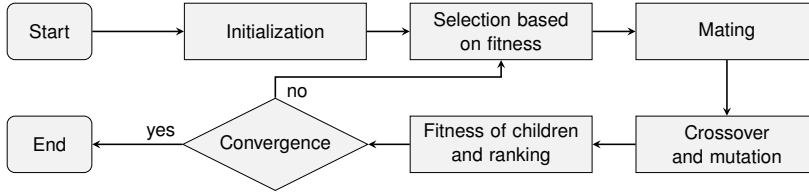
Figure 5.6: Flow chart showing the steps followed in the GA-based MOO.
