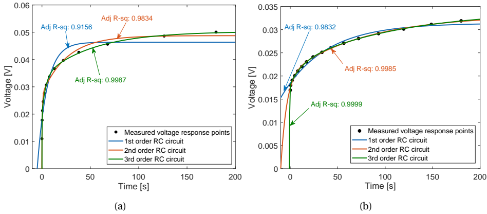
Figure A.7: Comparison of accuracy with modelling battery into different orders of RC circuits: (a) VRLA battery; (b) LFP battery.
