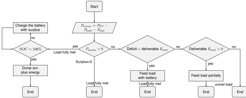
Figure 5.4: Flow chart explaining the power management scheme used in the standalone SHS model; it represents the algorithm followed in every time step. Note that dumped energy could be viewed as PV power production curtailment in practice, leading to potential under-utilization of solar energy.
