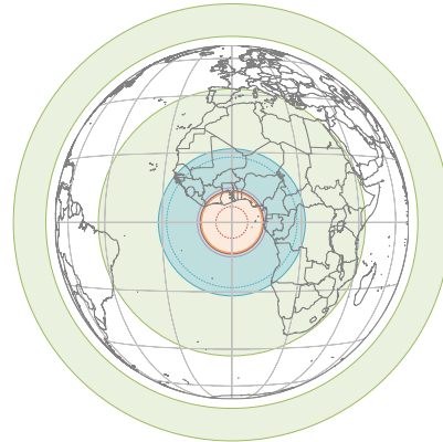
Fig. 8. Overlay of FoVs of NGSO satellites of Telesat LEO (blue), SpaceX Starlink (red), OneWeb LEO (orange), Astrome SpaceNet (purple) and Audacy (green). Dashed lines are the FoVs of the lowest altitude satellites in the constellation.
