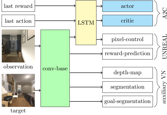
Fig. 1: A2CAT-VN neural network architecture.
