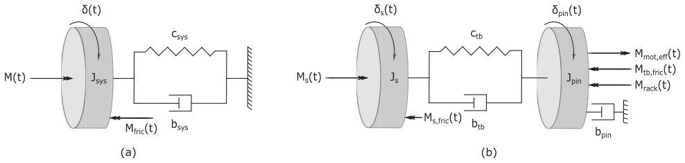
Figure 1. (a) A typical second-order mechanical inertia-spring-damper-friction model. (b) A simplified 2-DOF model of electric power assisted steering system, where M_{rack} represents the moment on the pinion (translated from steering rack force) originated from the vehicle model.
