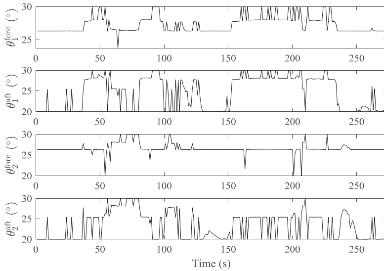
Figure 5.14: Angles between the towlines and the central line of the object.
