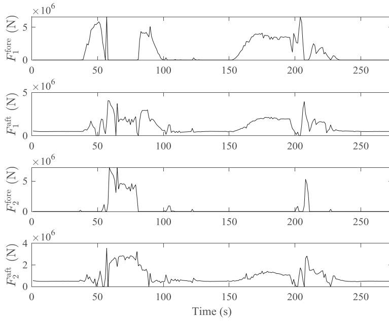
Figure 5.12: Forces along the towlines.
