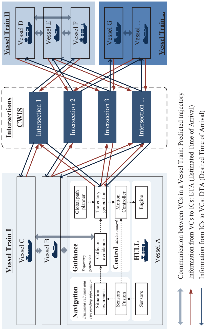
Figure 6.2: Cooperative Multi-Vessel System in urban waterway networks.
