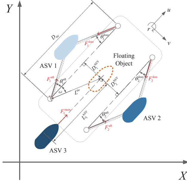
Figure 5.1: Configuration of the ASVs for cooperative object transport.
