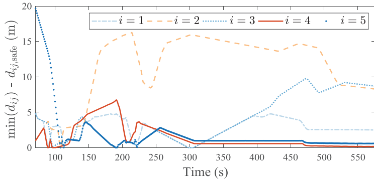
(b) Distance between an ASV and its nearest neighbor using Speed-based VTF.
