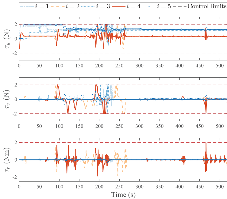
(b) Forces and moment of the ASVs using using Speed-based VTF.
