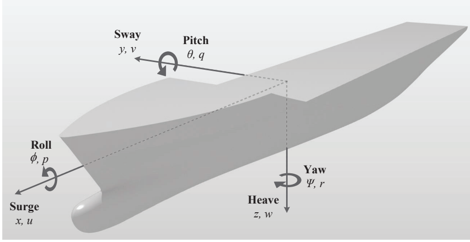
Figure 3.2: The body-fixed reference frame.
