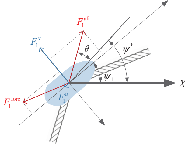
Figure 5.5: Force diagram of ASV 1.
