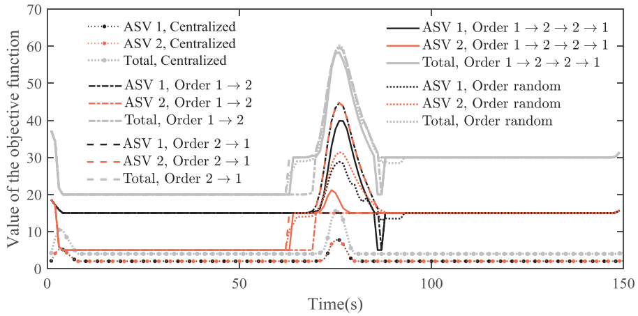
Figure 4.6: Objective value of each vessel with different updating sequences.
