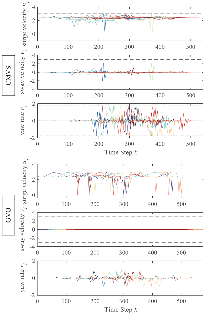
Figure 6.8: Linear and angular velocities of the ASVs that have the same dynamics with Delfia 1* using the proposed method and the GVO method. For the legend, see Figure 6.6.
