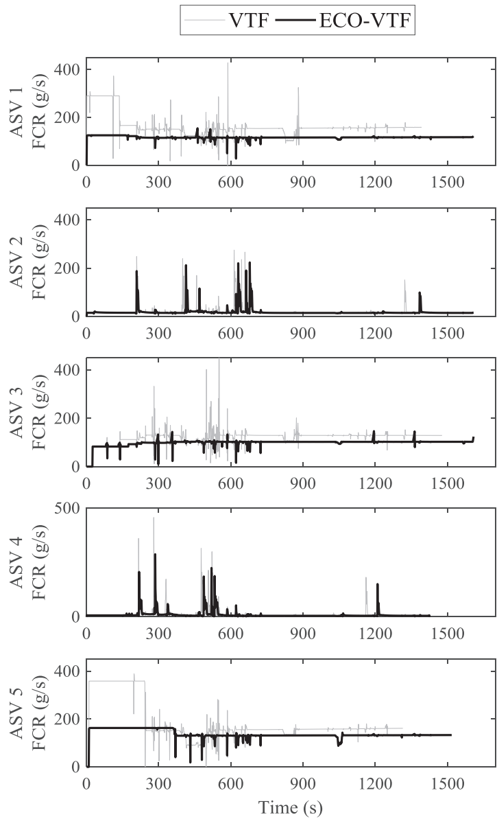
Figure 4.23: Fuel consumption rate of each ASV.
