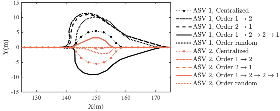
Figure 4.11: Trajectories of vessels using different responsibility parameters.
