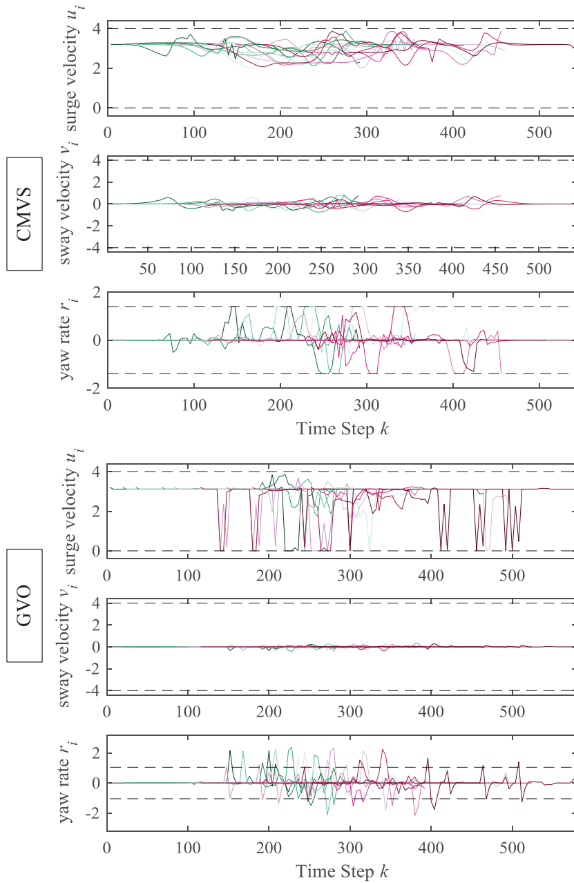
Figure 6.9: Linear and angular velocities of the ASVs that have the same dynamics with CyberShip 2 using the proposed method and the GVO method. For the legend, see Figure 6.6.
