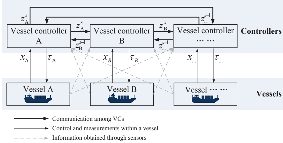
Figure 4.2: Control structure for VTF.
