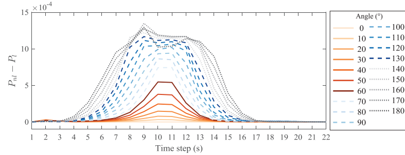
(b) Linearization error for each time step in Scenario 2.
