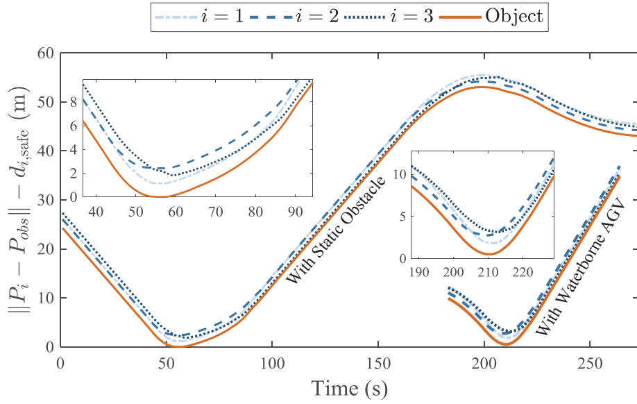
Figure 5.8: Distances with the static obstacle and the Waterborne AGV.
