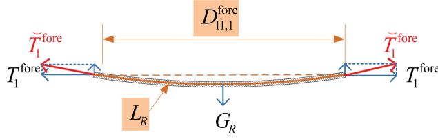
Figure 5.2: Tension on a towline.
