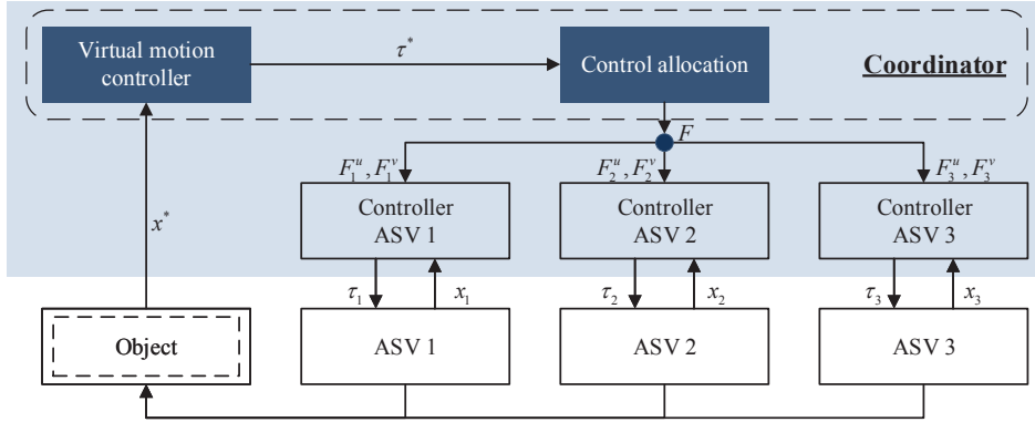
Figure 5.3: Multi-layer DMPC for cooperative object transport.
