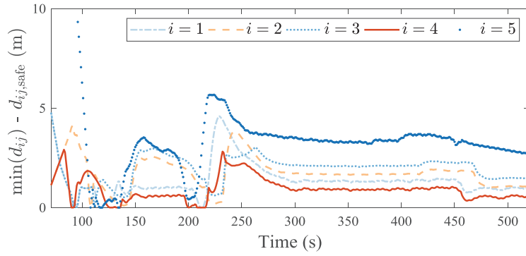
(a) Distance between an ASV and its nearest neighbor using Position-based VTF.
