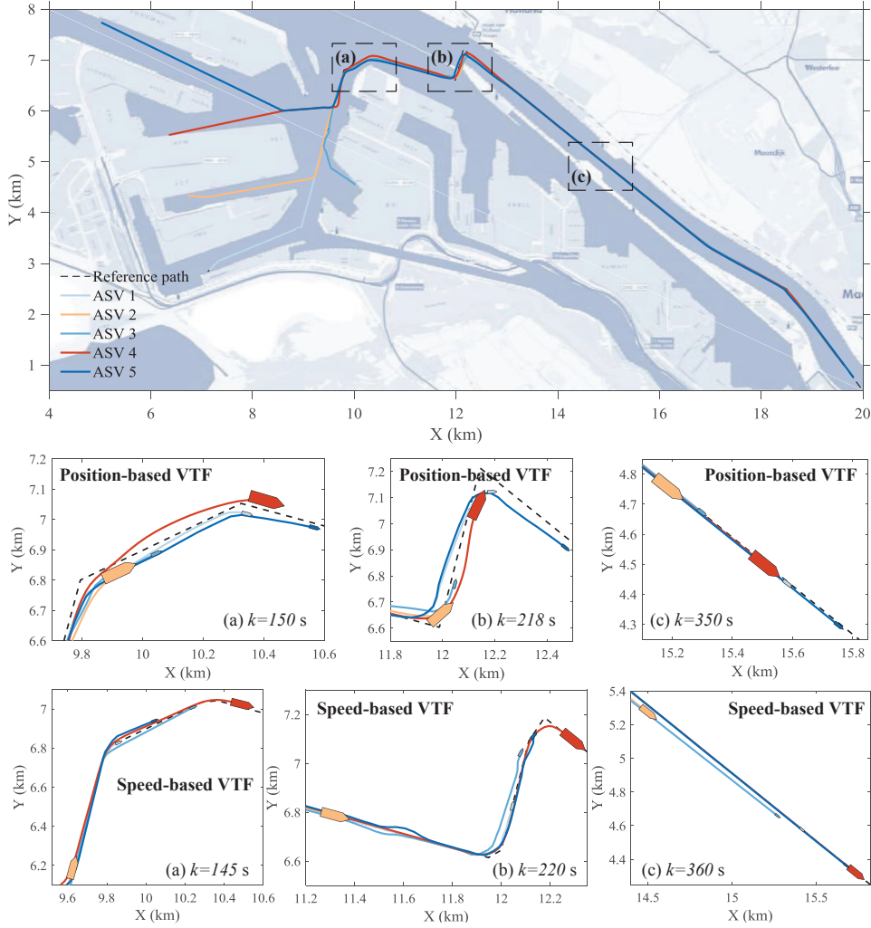
Figure 4.17: Trajectories of the ASVs.
