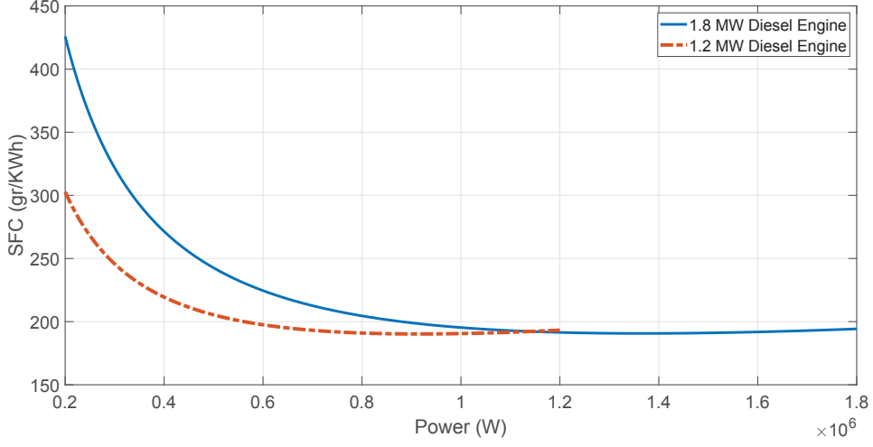
Figure 4.3: SFC curve of two diesel engines with different power ratings [27].
