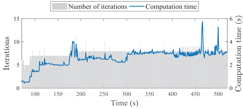
(b) Computation time and number of iterations using Speed-based VTF.
