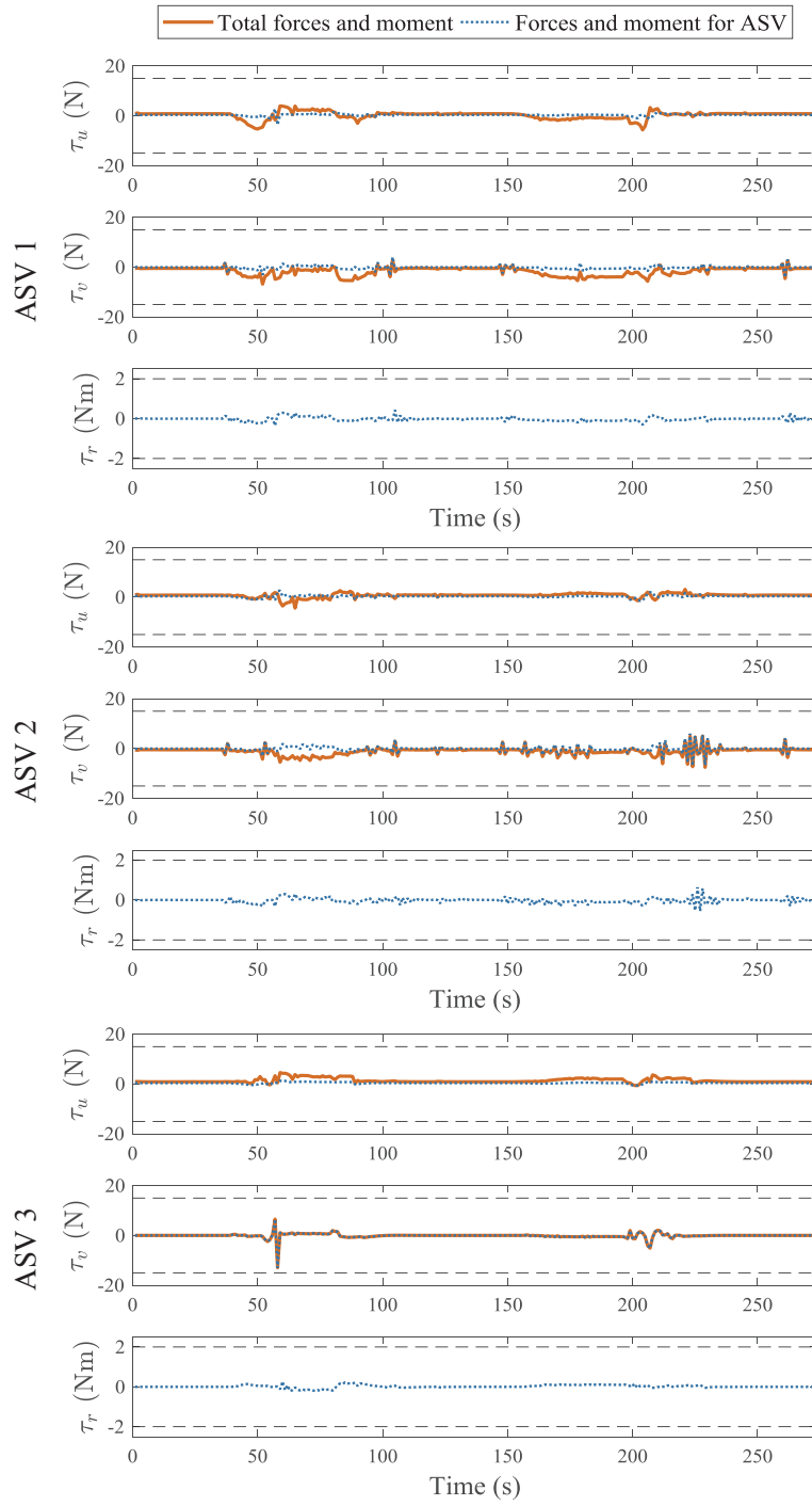
Figure 5.19: Forces and moment of each ASV with a time-varying configuration.
