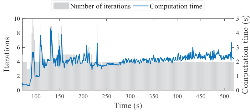
(a) Computation time and number of iterations using Position-based VTF.
