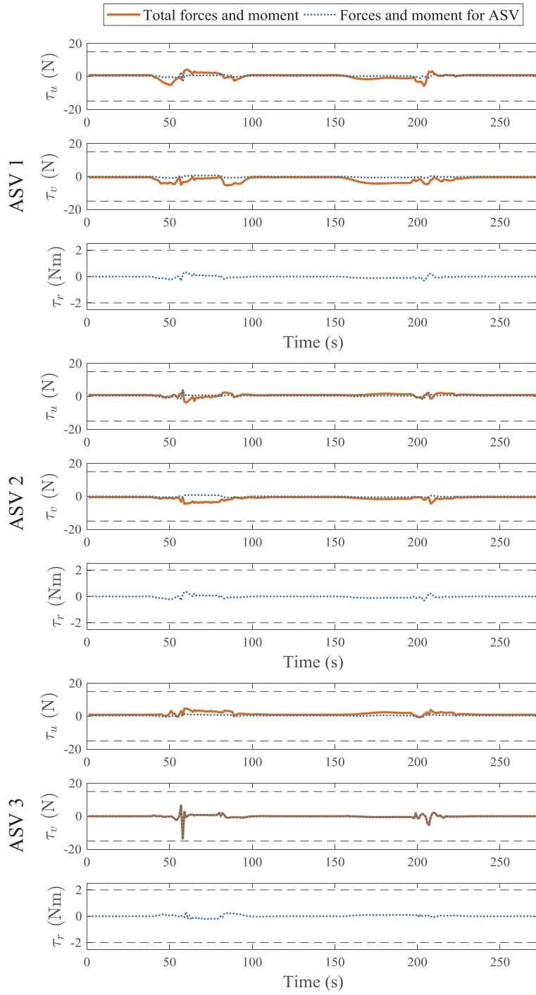
Figure 5.18: Forces and moment of each ASV with a constant configuration.
