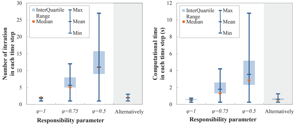
Figure 4.12: Number of iterations and computation time with different responsibility parameters.
