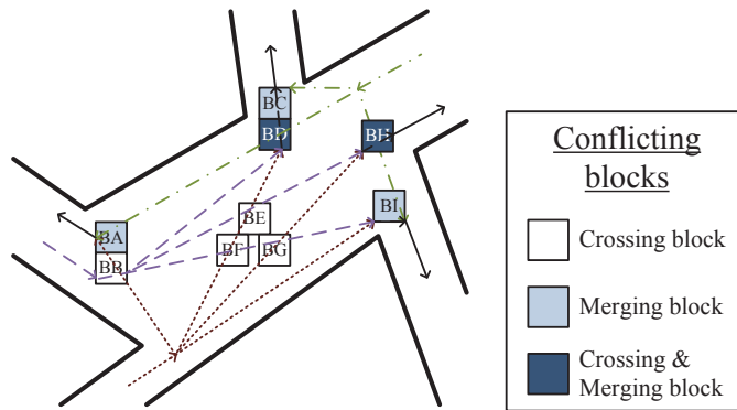
Figure 6.3: conflicting blocks at an intersection
