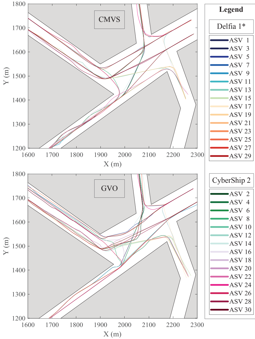
Figure 6.6: Comparison of the trajectories of ASVs using CMVS and GVO.
