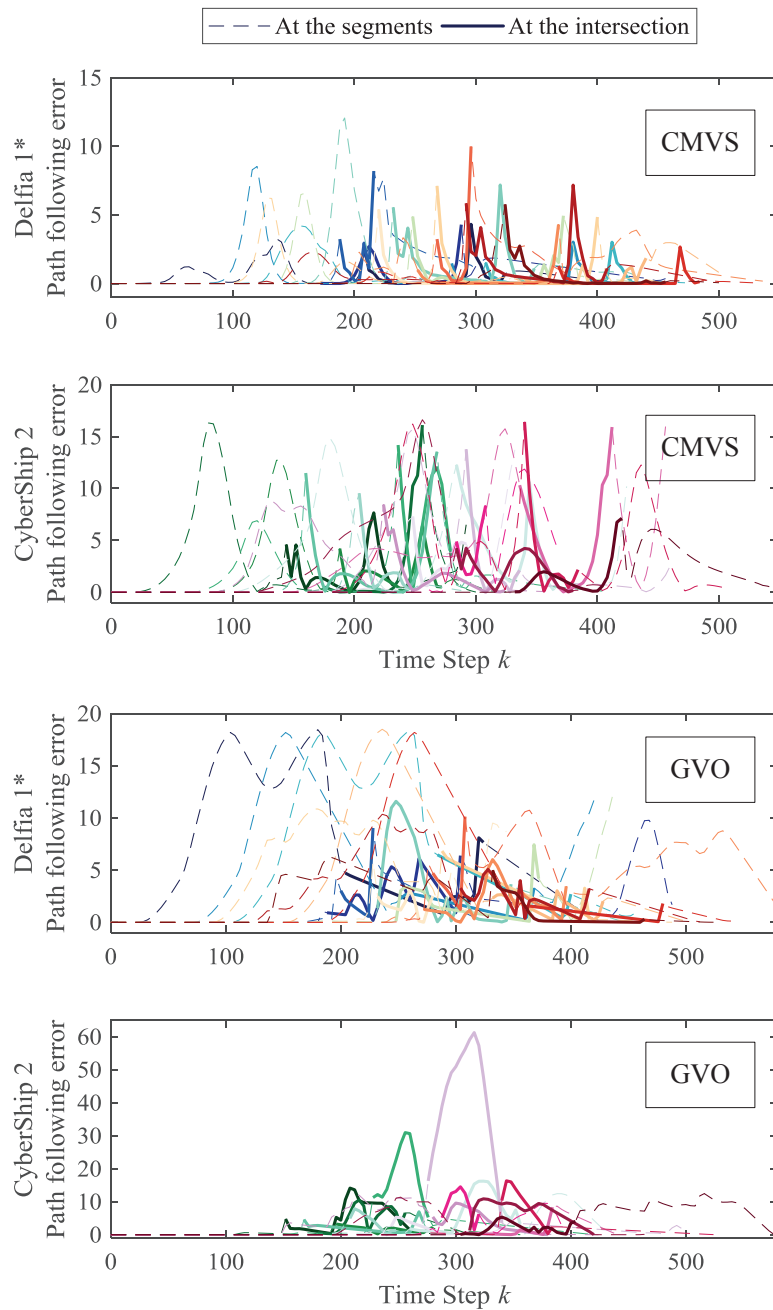
Figure 6.7: Comparison of path following errors of ASVs using CMVS and GVO. For the legend, see Figure 6.6.
