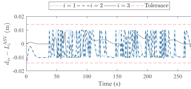
(b) Relative distance between ASVs and the object with a time-varying configuration.
