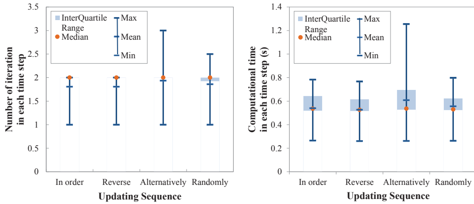
Figure 4.8: Number of iterations and computation time in each time step with different updating sequences 1 .
