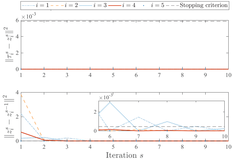
Figure 4.22: Primal and Dual Residual at time step k = 251 s using Position-based VTF.
