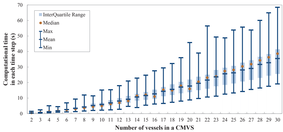
Figure 4.15: computation time when the number of vessels in a CMVS increases.
