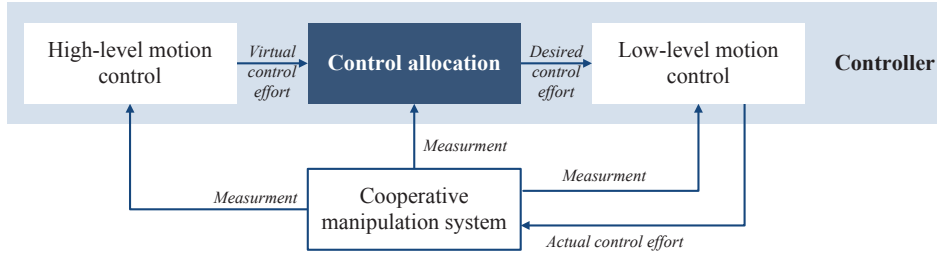
Figure 2.7: Generic control structure of cooperative manipulation.
