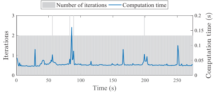
(a) Computation time and number of iterations with a constant configuration.
