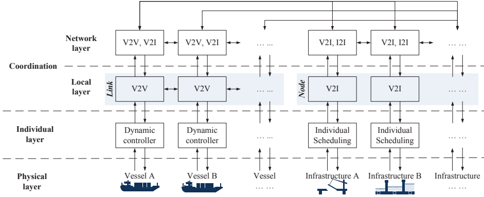
Figure 2.1: Hierarchical architecture of cooperations in waterborne transport systems.
