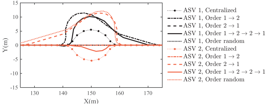
Figure 4.5: Trajectories of each vessel with different updating sequences.
