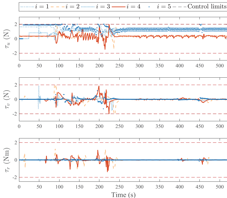
(b) Forces and moment of the ASVs using Position-based VTF.
