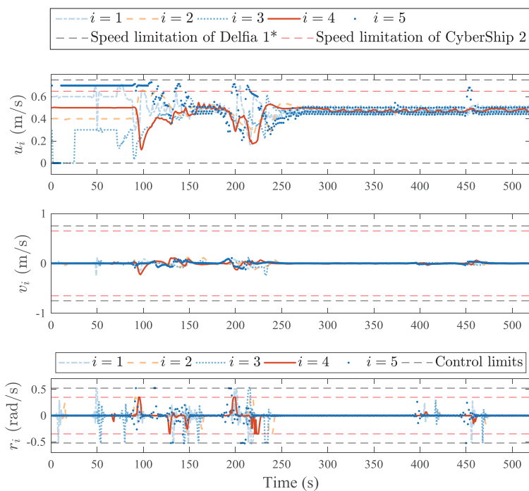
(a) Linear and angular velocities of the ASVs using Position-based VTF.
