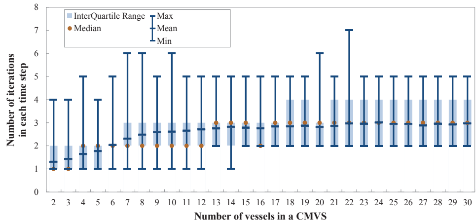
Figure 4.14: Number of iterations when the number of vessels in a CMVS increases.
