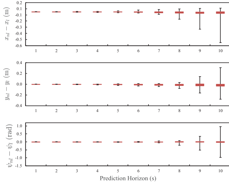
(b) Linearization errors over a prediction horizon in Scenario 2
