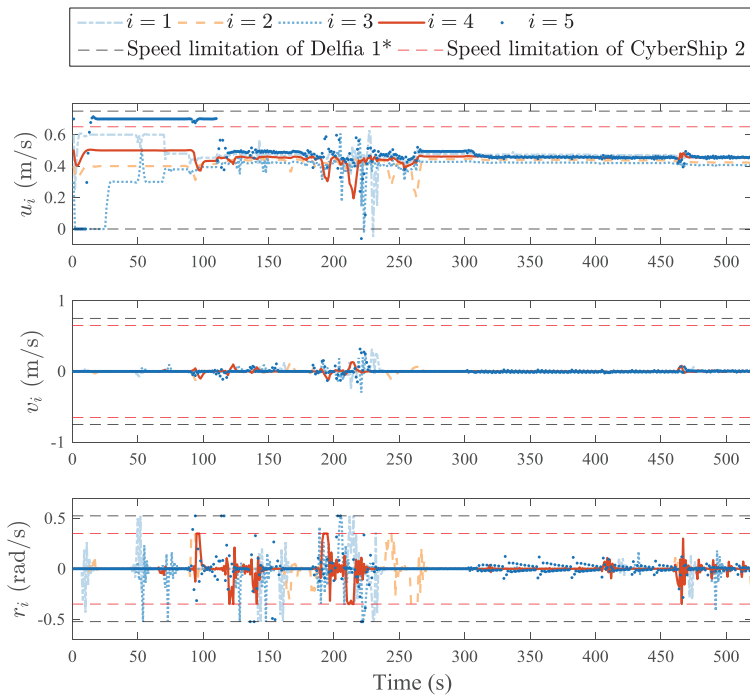
(a) Linear and angular velocities of the ASVs using Speed-based VTF.
