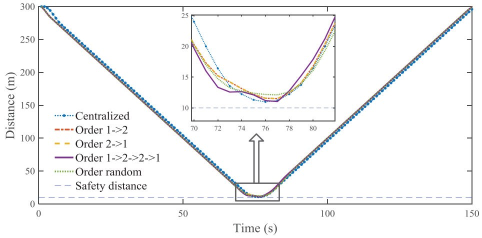
Figure 4.7: Relative distance with different updating sequences.
