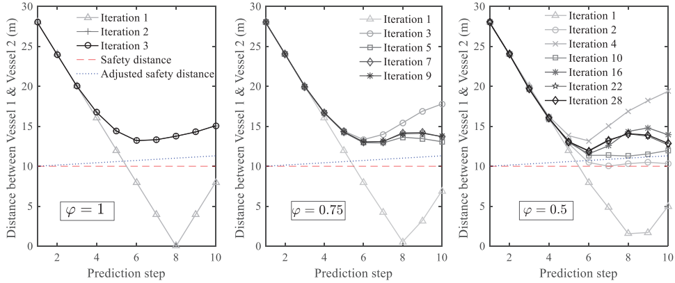
Figure 4.10: Predicted distance evolution.
