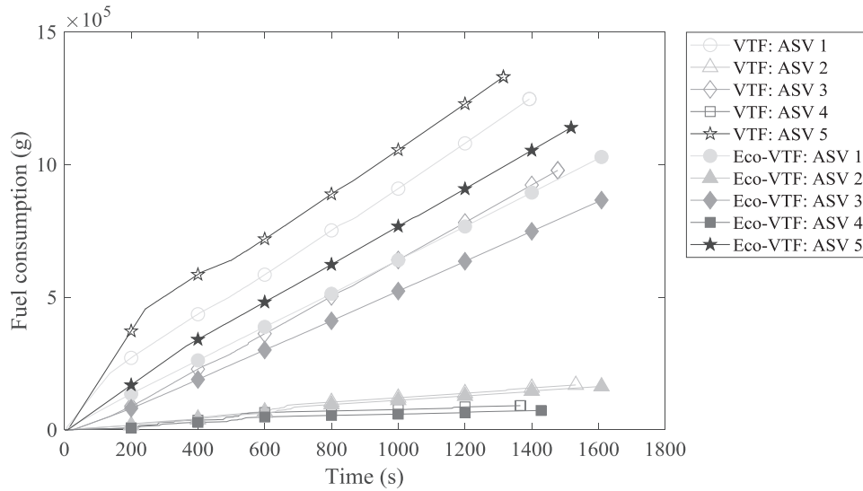
Figure 4.24: Total fuel consumption of each ASV.
