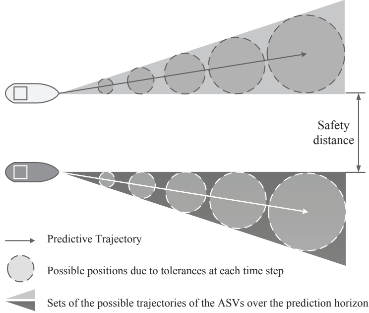
Figure 4.4: Adjustment on safety distance due to feasibility tolerances.
