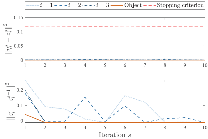
Figure 5.16: Evolution of the primal and dual residual at time step k = 124 s with a time-varying configuration.
