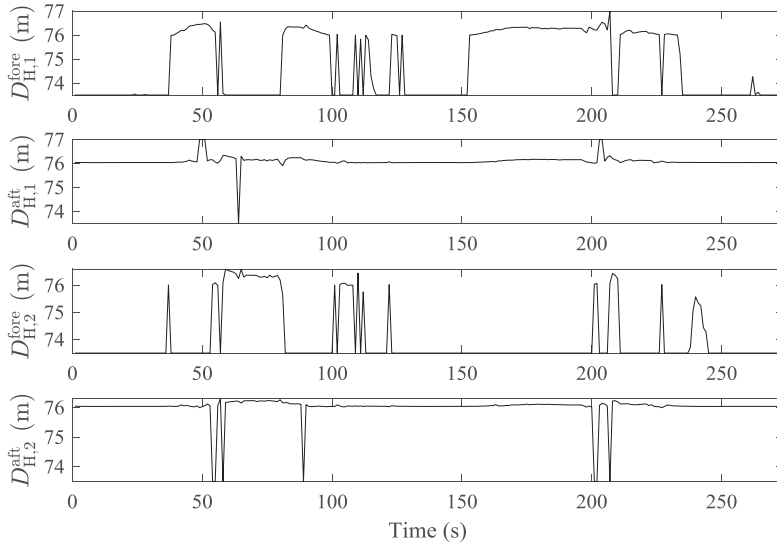
Figure 5.13: Horizontal distance between the two ends of each towline.
