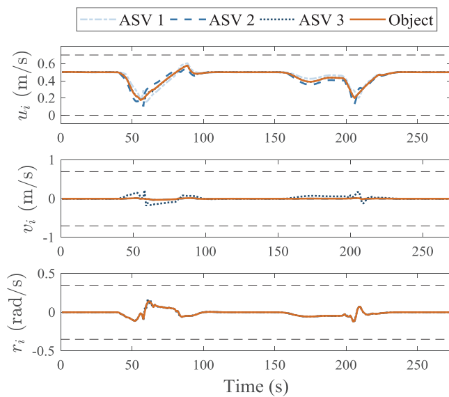
(a) Linear and angular velocities of the ASVs and the object with a constant configuration.
