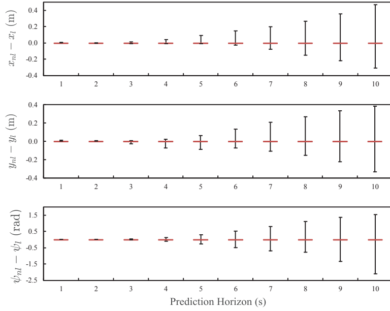
(a) Linearization errors over a prediction horizon in Scenario 1
