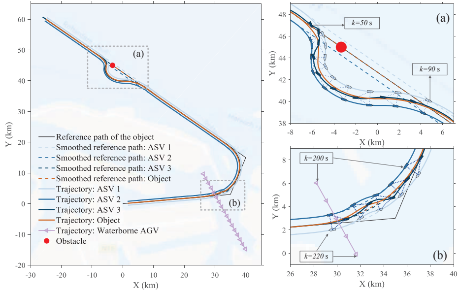
Figure 5.7: Trajectories of the ASVs and the object.
