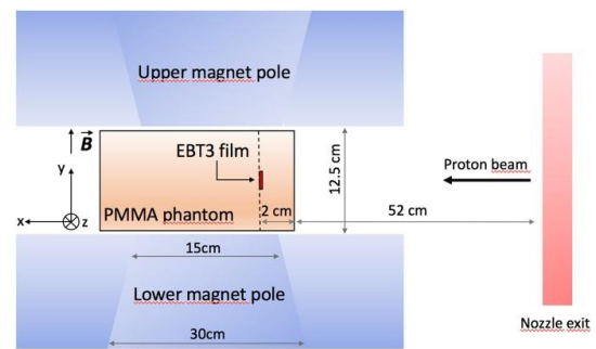
Fig. 1 Sketch view of the experimental setup used for the EBT3 films calibration.
