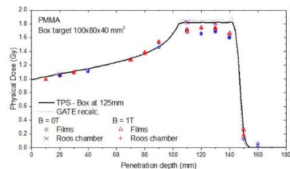
Fig. 2 Spread out Bragg peak measured without/within a magnetic field region. The continue and dash lines correspond to the planned and MC-recalculated dose distributions respectively.
