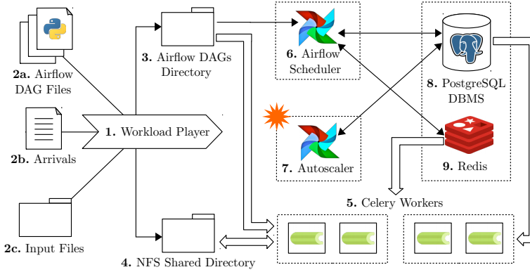
Figure 5.1: System architecture.
