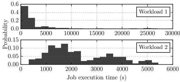
Figure 4.7: The distribution of job execution times in the workloads (all the axes have different scales).
