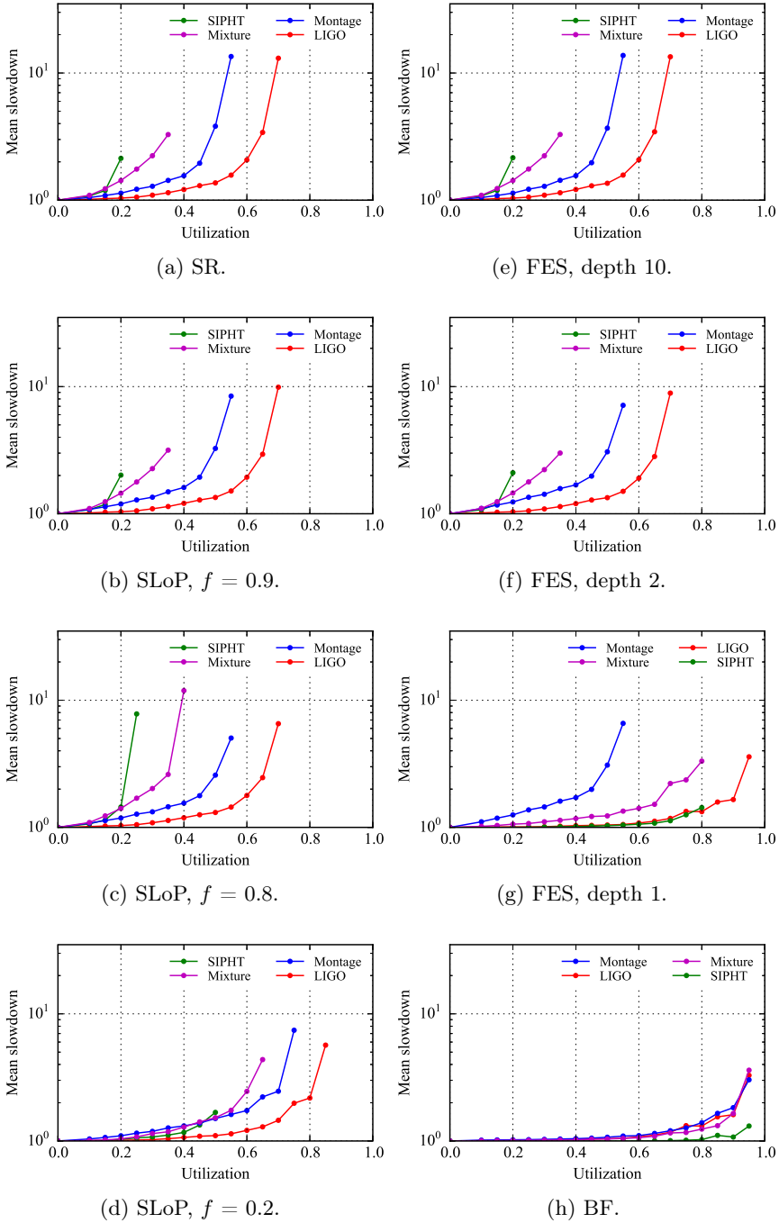
Figure 2.5: The mean slowdown of workflows as a function of the utilization for the different policies and for each of the four workload types (the vertical axis is in log scale).
