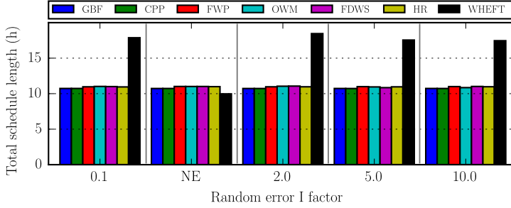
Figure 3.8: The total schedule length in hours of a batch submission based on Workload I with 1000 workflows in a homogeneous system. NE stands for No Error.
