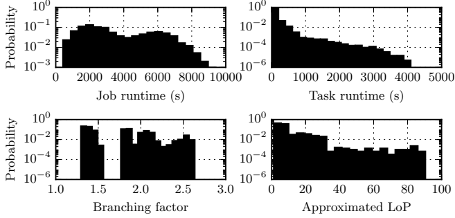
Figure 3.1: Statistical characteristics of Workload I. The vertical axes have a log scale.
