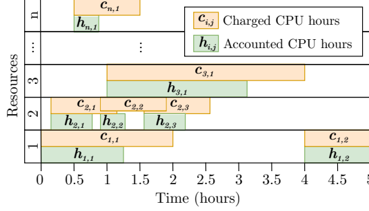
Figure 4.3: The difference between accounted and charged CPU hours.
