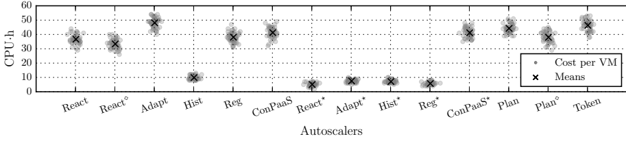
Figure 4.17: Charged cost in CPU hours for the autoscalers running Workload 1. For each policy, per VM costs are displayed with a slight random horizontal shift to avoid excessive superimposing.
