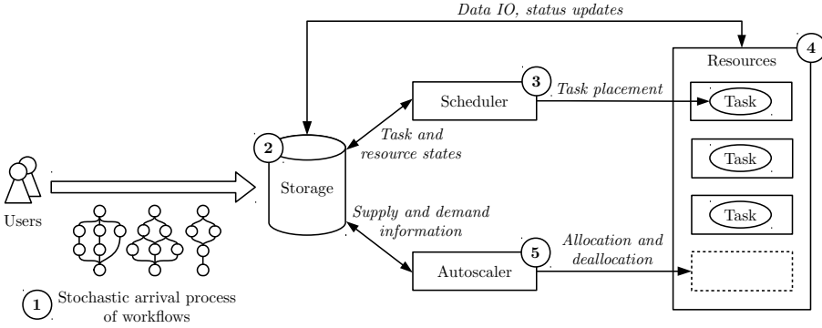
Figure 1.3: The general architecture of a workflow management system for online workflow scheduling.
