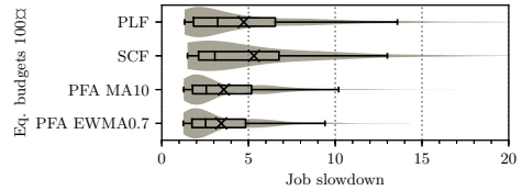
Figure 5.7: Variability of job slowdowns for all the studied autoscalers with equal budgets for both users when running WL II. PFA autoscaler was executed with MA depth 10 and EWMA with pole value 0.7. Means are marked with \times .
