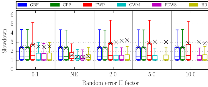
(c) Random error II, Workload I.
