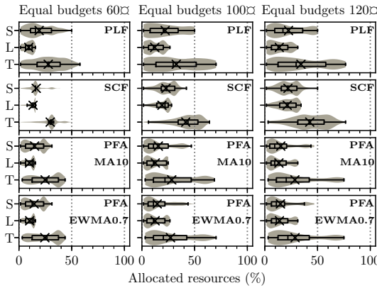
Figure 5.14: Variability of allocated resources for User 1 for the studied autoscalers with equal budgets of 60, 100, 120 when running WL I. For Small and Large resource types, and in Total. Means are marked with \times .
