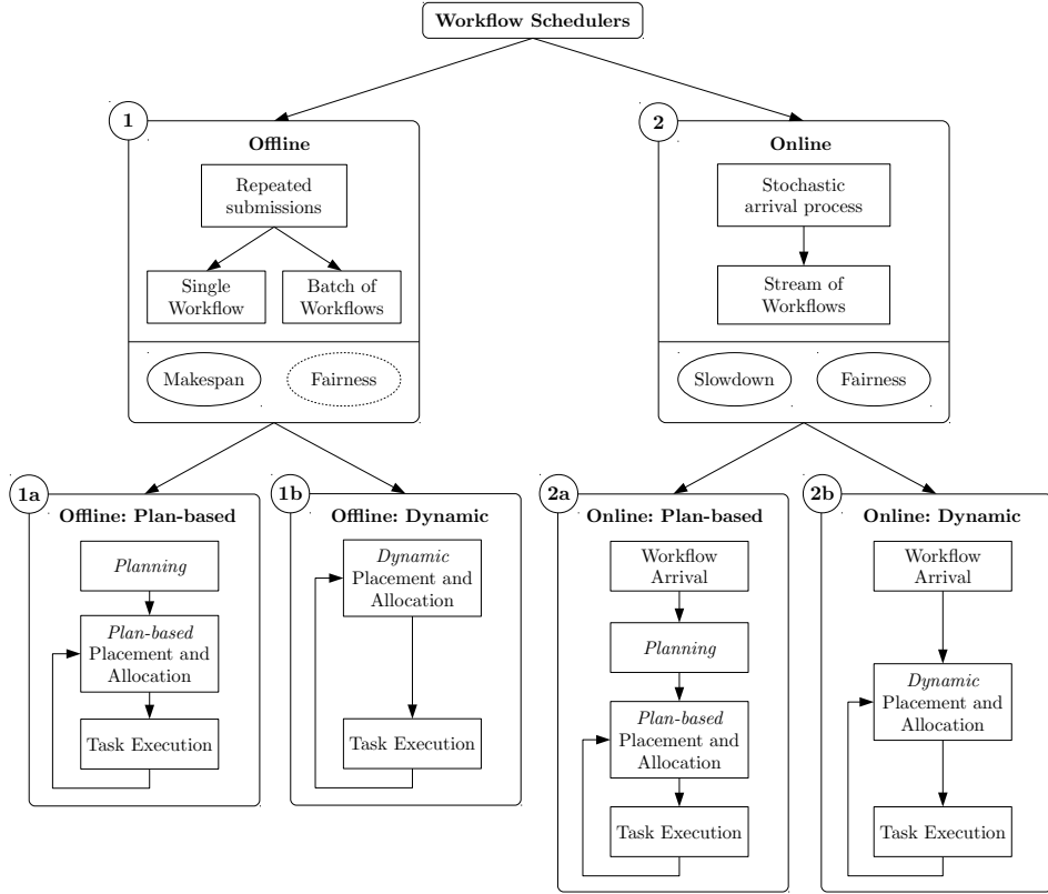
Figure 1.2: A hierarchy of classes of workflow scheduling approaches for task placement and resource allocation.
