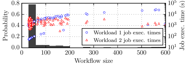
Figure 4.5: The distribution of job sizes in the workloads (histogram, left vertical axis) and the dependency between the job size and its execution time (points, right vertical axis). The right vertical axis is in log scale.
