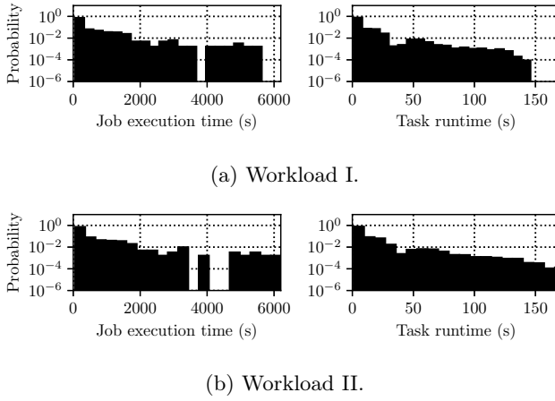
Figure 5.2: Statistical characteristics of the workloads. The vertical axes have a log scale.
