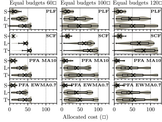
Figure 5.8: Variability of monetary cost for allocated resources per billing interval for User 1 for the studied autoscalers with equal budgets of 60$, 100$, and 120$ when running WL I. For Small and Large resource types, and in Total. Means are marked with \times .
