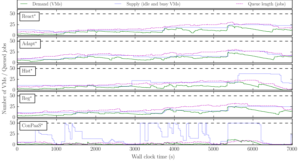
Figure 4.9: The experimental dynamics of all the five considered general autoscaling policies (Workload 1, service rate 14.0) during the cropped interval of 7,000 s. The horizontal dashed line indicates the resource limit of 50 VMs.
