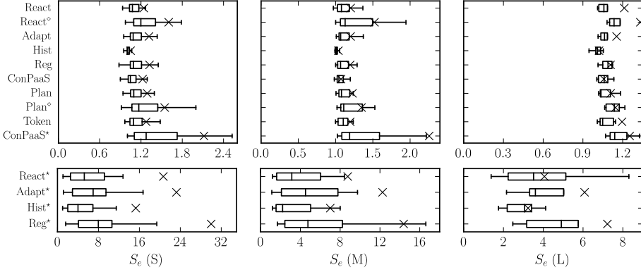
Figure 4.15: Variability of elastic slowdowns for (S) small, (M) medium, and (L) large workflow sizes in Workload 1. Means are marked with \times . The horizontal axes have different scales.
