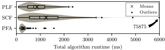
Figure 5.3: Variability of total runtimes for all the considered autoscalers.
