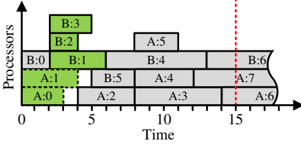
(b) Unlimited partial plan.
