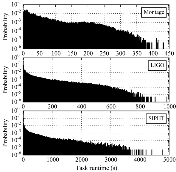
Figure 2.4: The distribution of the task runtimes for each workflow type (the horizontal axes have different scales, and the vertical axes are in log scale).
