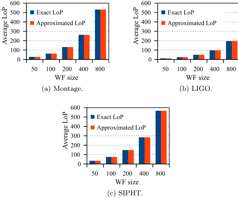
Figure 2.2: A comparison of the exact and the approximation method for calculating the LoP for different workflow structures.
