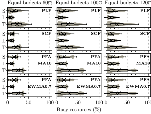
Figure 5.12: Variability of busy resources for User 1 for the studied autoscalers with equal budgets of 60, 100, 120 when running WL I. For Small and Large resource types, and in Total. Means are marked with \times .
