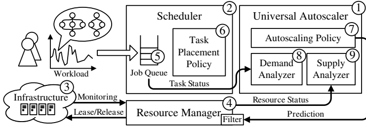
Figure 4.1: Elastic cloud platform.
