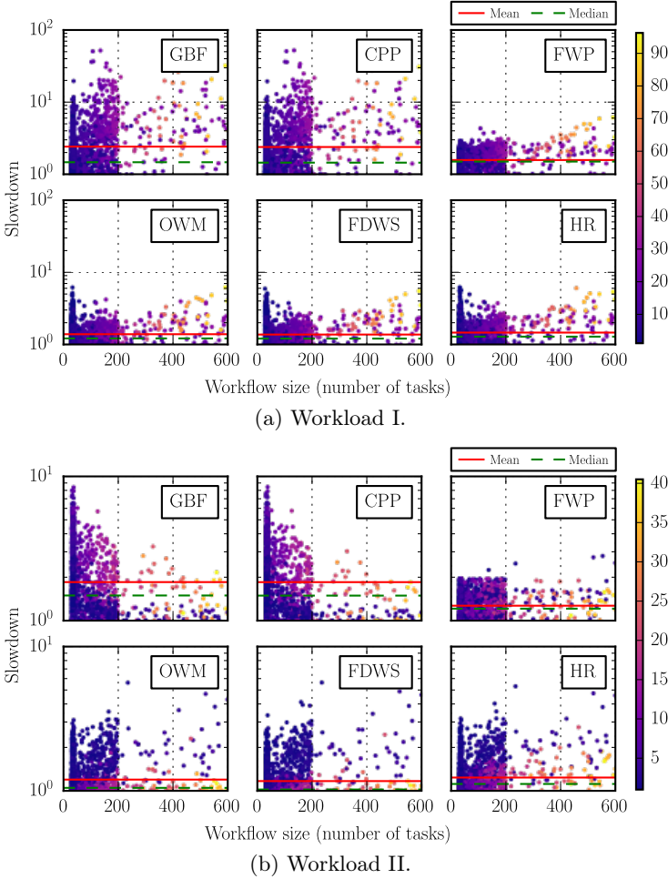
Figure 3.9: Scatter plots of slowdowns versus the sizes of workflows at 98% utilization in a homogeneous system without an error. The point color encodes the approximated LoP, the vertical axes have a log scale.
