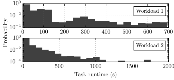
Figure 4.6: The distribution of task runtimes in the workloads (the horizontal axes have different scales, and the vertical axes are in log scale).
