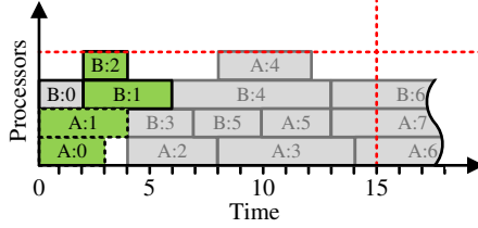
(c) Limited partial plan.
