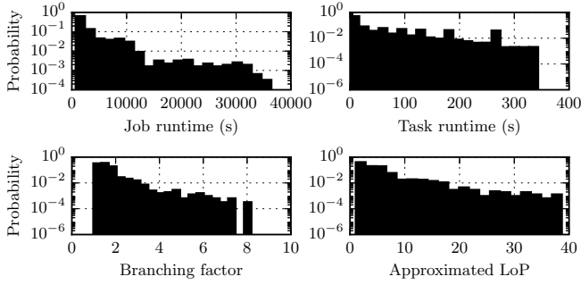
Figure 3.2: Statistical characteristics of Workload II. The vertical axes have a log scale.
