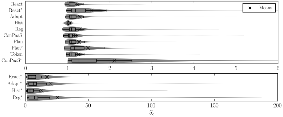
Figure 4.14: Variability of elastic slowdowns for all the workflows in Workload 1. Values in wider parts of shaded areas are more probable than those in narrower parts. The horizontal axes have different scales.
