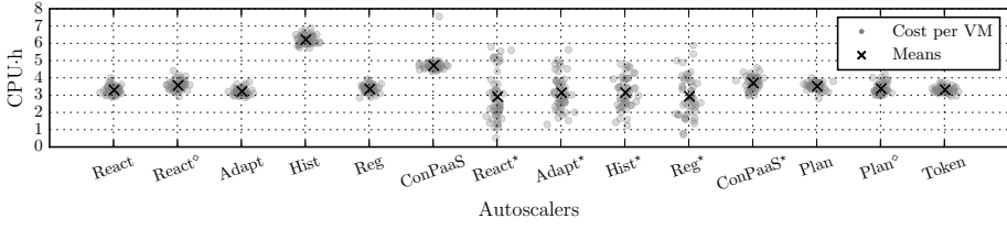
Figure 4.16: Accounted cost in CPU hours for all the considered autoscalers running Workload 1. For each policy, per VM costs are displayed with a slight random horizontal shift to avoid excessive superimposing.
