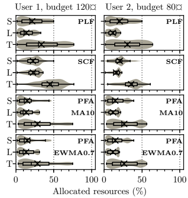
Figure 5.15: Variability of allocated resources for each user with different budgets 120 and 80 when running WL I. For Small and Large resource types, and in Total. Means are marked with \times .
