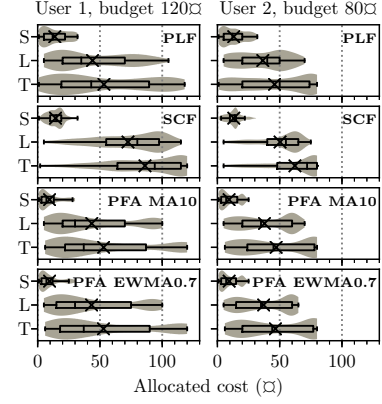
Figure 5.9: Variability of monetary cost for allocated resources per billing interval for each user for the studied autoscalers with different budgets when running WL I. For Small and Large resource types, and in Total. Means are marked with \times .
