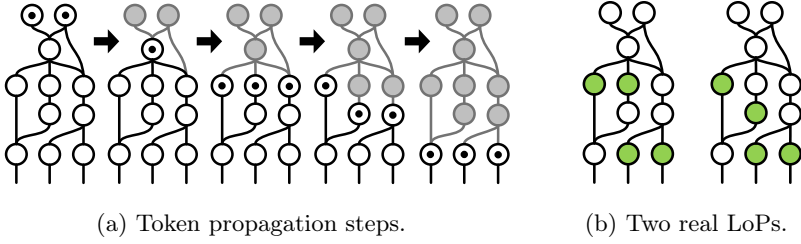
Figure 2.1: An example of LoP approximation (a) versus the exact LoP (b).
