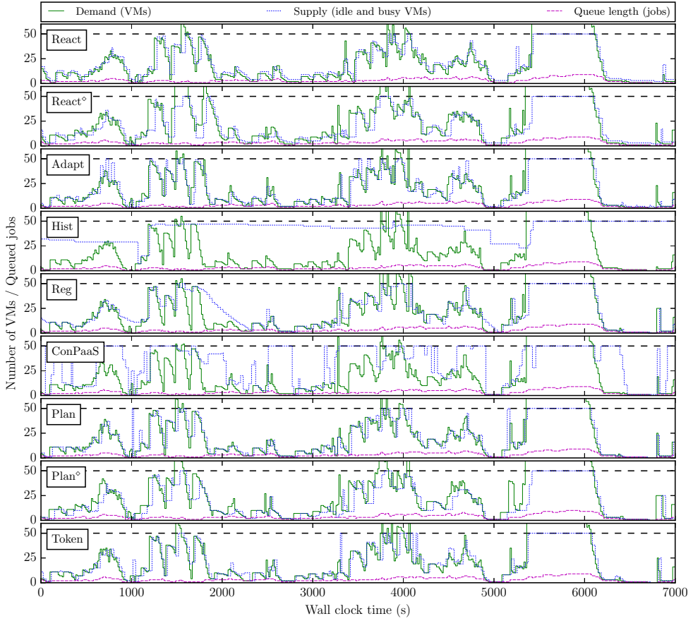
Figure 4.8: The experimental dynamics of five general autoscaling policies (Workload 1, service rate 1.0) and two workflow-specific policies during the cropped period of 7,000 s. The horizontal dashed line indicates the resource limit of 50 VMs. The diamond symbol ( \diamond ) marks the experiments where the VM booting time is longer than the autoscaling interval.
