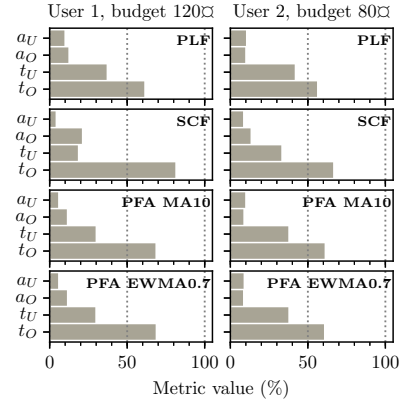
Figure 5.11: Elasticity metrics for each user for the studied autoscalers with different budgets 120$ and 80$ when running WL I. For all the metrics lower values are better.
