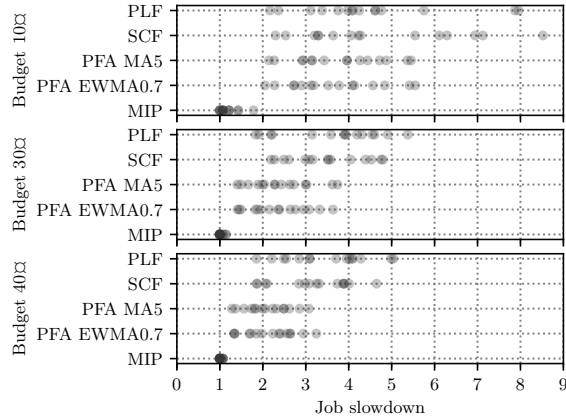
Figure 5.18: The variability of job slowdowns for different budgets for Airflow-based and MIP results.
