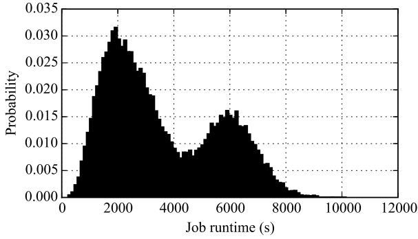
Figure 2.3: The distribution of the total workflow execution times in the workloads.
