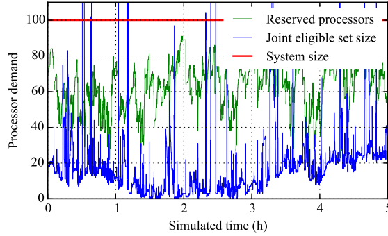
Figure 2.7: The dynamics of the joint eligible set size and the number of reserved processors during the simulation of the SR policy at a utilization of 0.35 during a 5-hour period.
