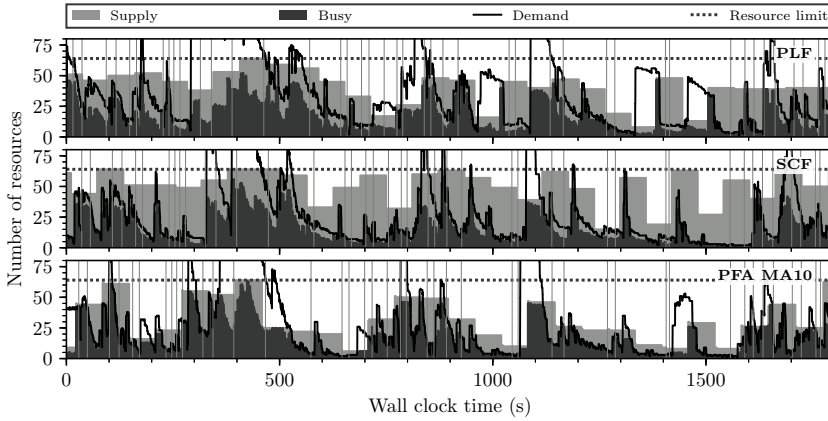
Figure 5.16: The dynamics of autoscaling on a cropped interval of 1,800 seconds for both users with equal budgets 120 \square . Vertical lines indicate workflow arrivals.
