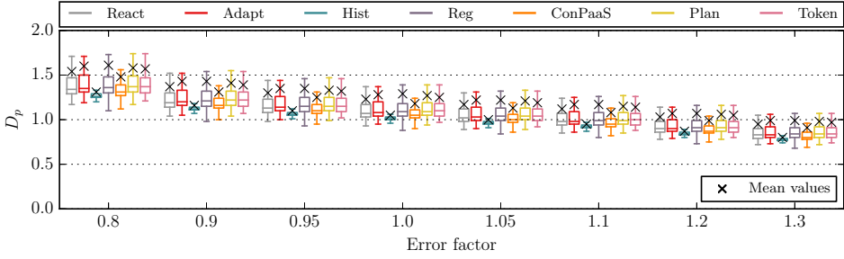
Figure 4.12: The effect of changing enforced per-workflow deadlines on the deadline proximity ratio (for all workflows in Workload 1).
