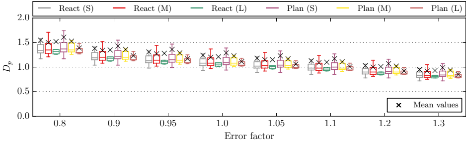
Figure 4.13: The effect of changing enforced per-workflow deadlines on the deadline proximity ratio for React and Plan autoscalers plotted separately for (S) small, (M) medium, and (L) large workflow sizes in Workload 1.
