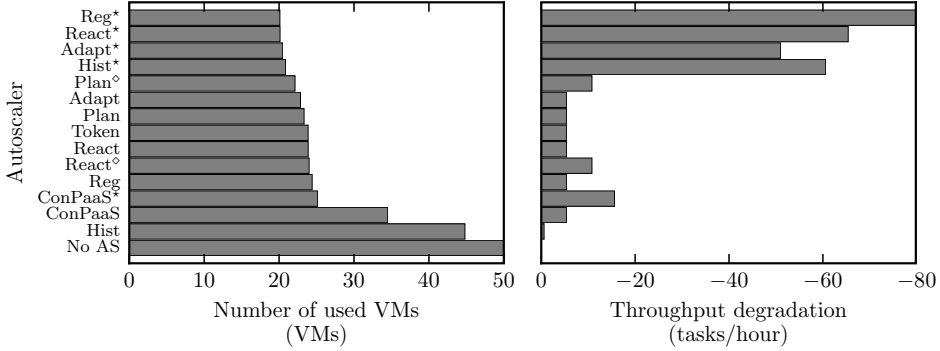
Figure 4.10: The average number of used VMs during the experiment and the average throughput degradation (compared with the no autoscaler case). All results are given for Workload 1.
