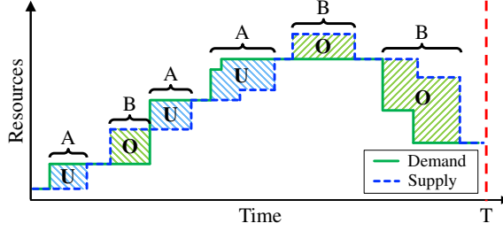
Figure 4.2: The supply and demand curves illustrating the under- and over-provisioning periods (A and B) quantified in the number of resources (areas U and O).
