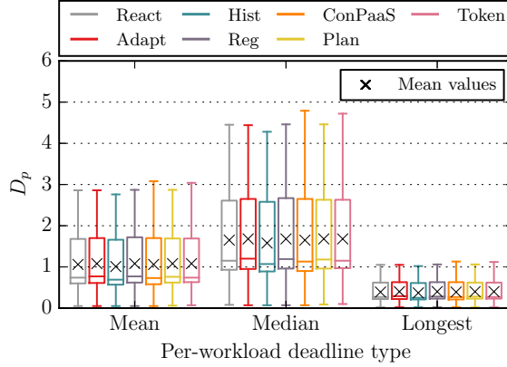
(a) All autoscalers and all workflows.
