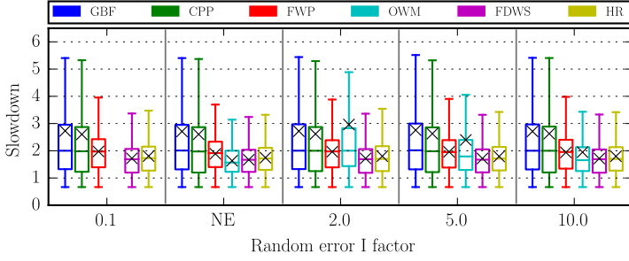
(a) Random error I, Workload I.
