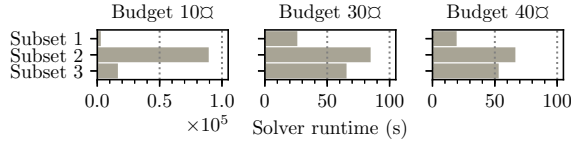
Figure 5.17: Solver runtimes for all three subsets of workflows with different budget constraints. In the left plot the x axis has much larger scale than in the other two plots.
