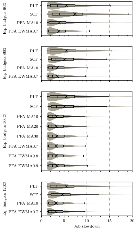
Figure 5.5: Variability of job slowdowns for all the studied autoscalers with equal budgets of 60, 80, 100, and 120 when running WL I. PFA autoscaler was executed with different smoothing methods. Means are marked with \times .
