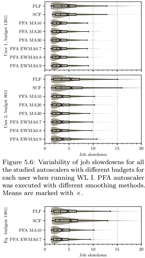
Figure 5.7: Variability of job slowdowns for all the studied autoscalers with equal budgets for both users when running WL II. PFA autoscaler was executed with MA depth 10 and EWMA with pole value 0.7. Means are marked with \times .
