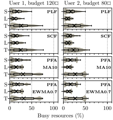
Figure 5.13: Variability of busy resources for each user with different budgets 120 and 80 when running WL I. For Small and Large resource types, and in Total. Means are marked with \times .
