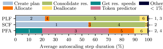
Figure 5.4: Average duration of each algorithm step within the total algorithm runtime for each considered autoscaler. The superimposed numbers represent corresponding algorithm steps.
