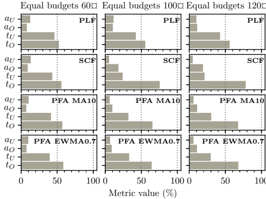
Figure 5.10: Elasticity metrics for User 1 for the studied autoscalers with equal budgets of 60$, 100$, 120$ when running WL I. For all the metrics lower values are better.
