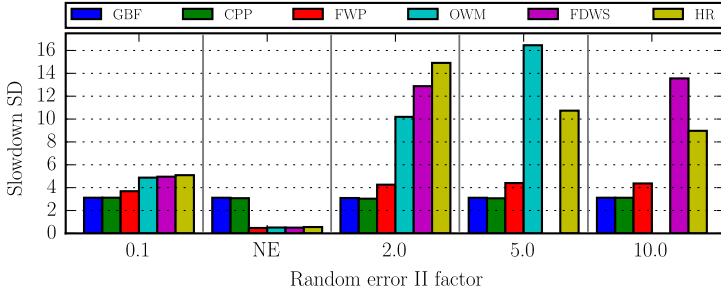
(c) Random error II, Workload I. The vertical axis has larger scale.
