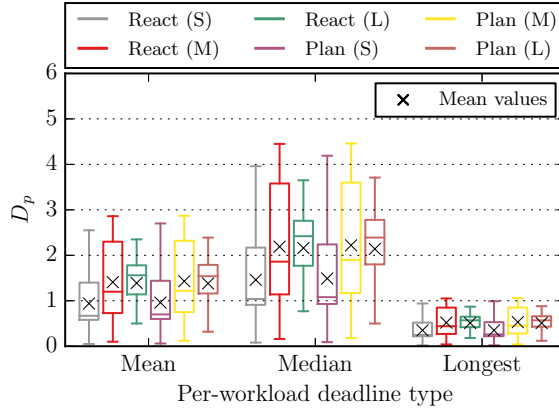
(b) React and Plan autoscalers, (S) small, (M) medium, and (L) large workflow sizes.
