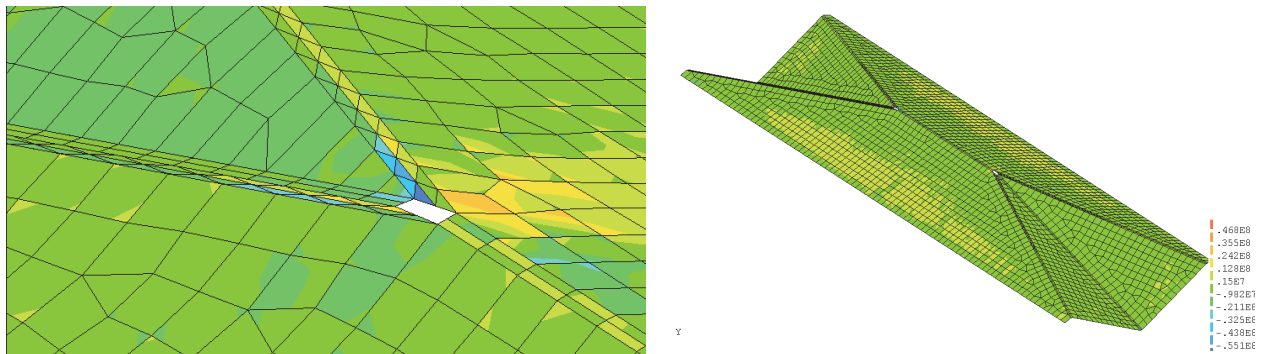
Fig. 28,29 Graphically represented principle stresses S2 results of the finite element analysis applying selfweight and windload
