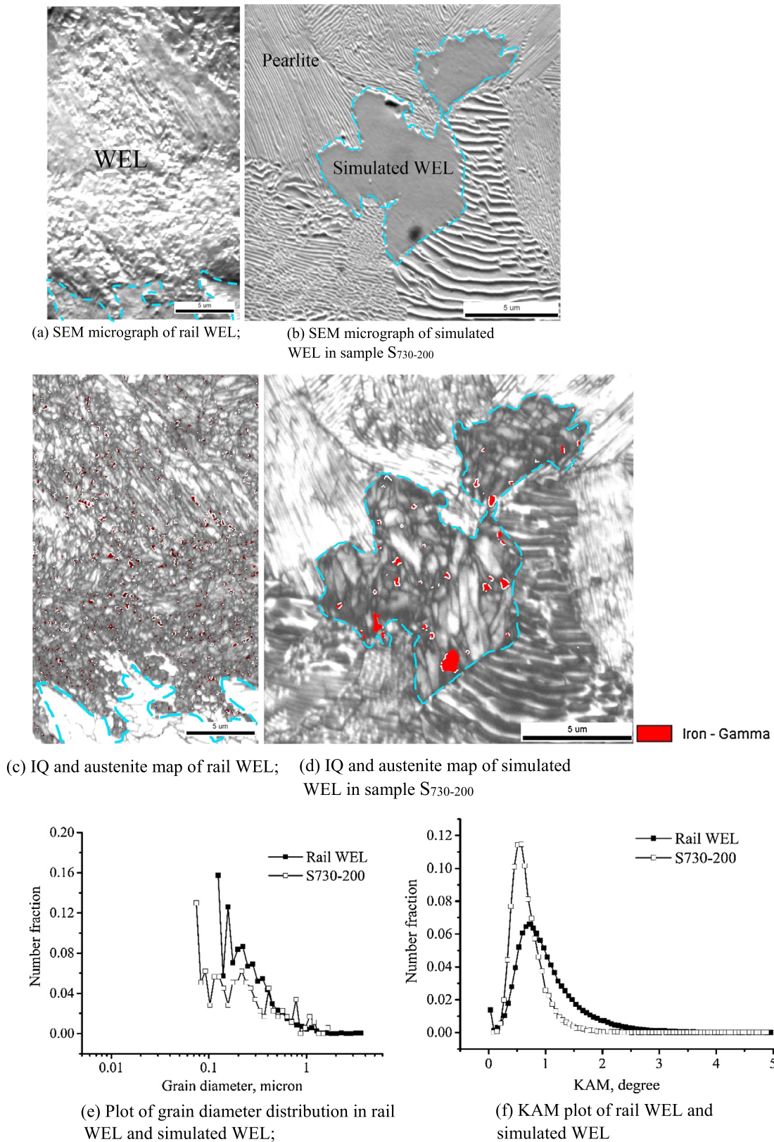
Fig. 5. (a) SEM micrograph of rail WEL. The blue lines indicate the WEL/pearlite boundary; (b) the SEM micrograph of the simulate WEL in sample S730-200; (c) the IQ map of rail WEL in (a), imposed with austenite phase map. The phase boundaries satisfying the K-S orientation relationship are delineated by the white lines; (d) the IQ map of laboratory WEL of specimen S730-200 in (b), imposed with austenite phase map; (e) grain diameter distribution of both rail WEL and laboratory WEL in S730-200; (f) KAM distribution of both rail WEL and laboratory WEL in S730-200. (For interpretation of the references to colour in this figure legend, the reader is referred to the web version of this article.)
