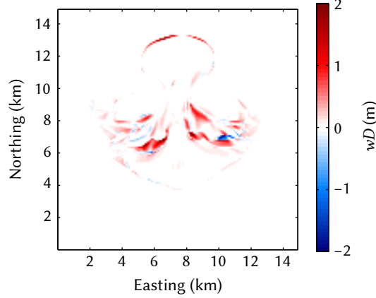
Figure 4.5: Weighted displacements wD for the prediction at 0^\circ . Here D = \sqrt{(B_x^2 + B_y^2)} is the field of displacement magnitudes computed from the backward displacement vector field \mathbf{B} (see Eq. 4.1) and w is determined according to Eq. 4.2.
