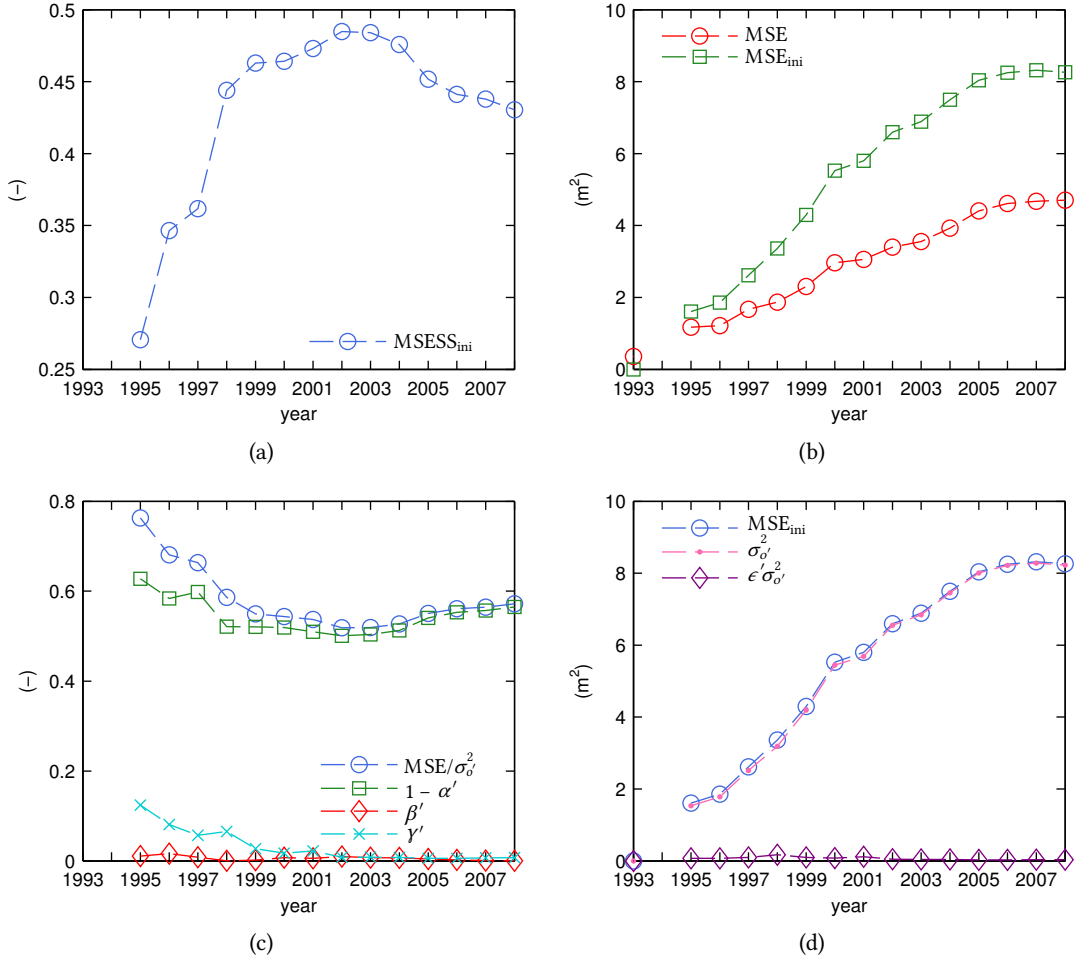
Figure 2.6: Model performance for Bornrif: (a) MSE skill score with the zero change model as the reference, \text{MSESS}_{\text{ini}} , (b) MSE of the computations and \text{MSE}_{\text{ini}} of the initial bed (zero change reference model), (c) MSE normalized with the variance of the cumulative observed bed changes and its decomposition, Eqs. 2.6 and 2.7 and (d) \text{MSE}_{\text{ini}} and its decomposition, Eqs. 2.8 and 2.9.
