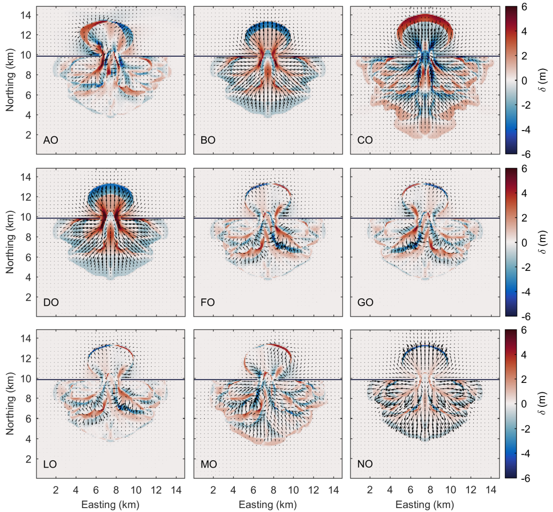
Figure 5.10: Bed level differences and transport fields, with the length and direction of the arrows indicative of the transport magnitude and direction, respectively, for predictions A through N compared to the “observations” O.
