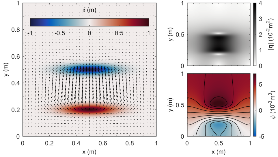
Figure 5.4: Optimal solution, with closed boundaries, for prediction 3. Left panel: bed level difference \delta = h_1 - h_2 with the arrows indicating the transport field (length and direction of arrows indicative of the transport magnitude and direction, respectively). Right panels: transport field represented by the transport magnitude ( top ) and potential \phi ( bottom ).
