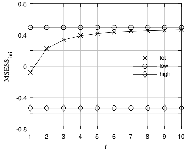
Figure 3.8: Variation of \text{MSESS}_{\text{ini}} in time for the low-frequency ( low ) and high-frequency ( high ) part as well as for the combined signal ( tot ).
