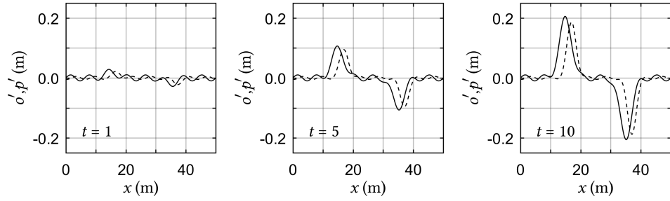
Figure 3.7: Measured (solid lines) and predicted anomalies at three moments ( t = 1, 5 and 10 ) in the simulation, consisting of a constant high-frequency part and a low-frequency part that increases in magnitude in time.
