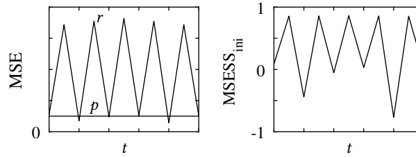
Figure 3.6: Skill for a hypothetical seasonal system. Left : the MSE for the prediction p is constant in time and the MSE_r of the zero change reference prediction r fluctuates. Right : the MSESS_{ini} also fluctuates.
