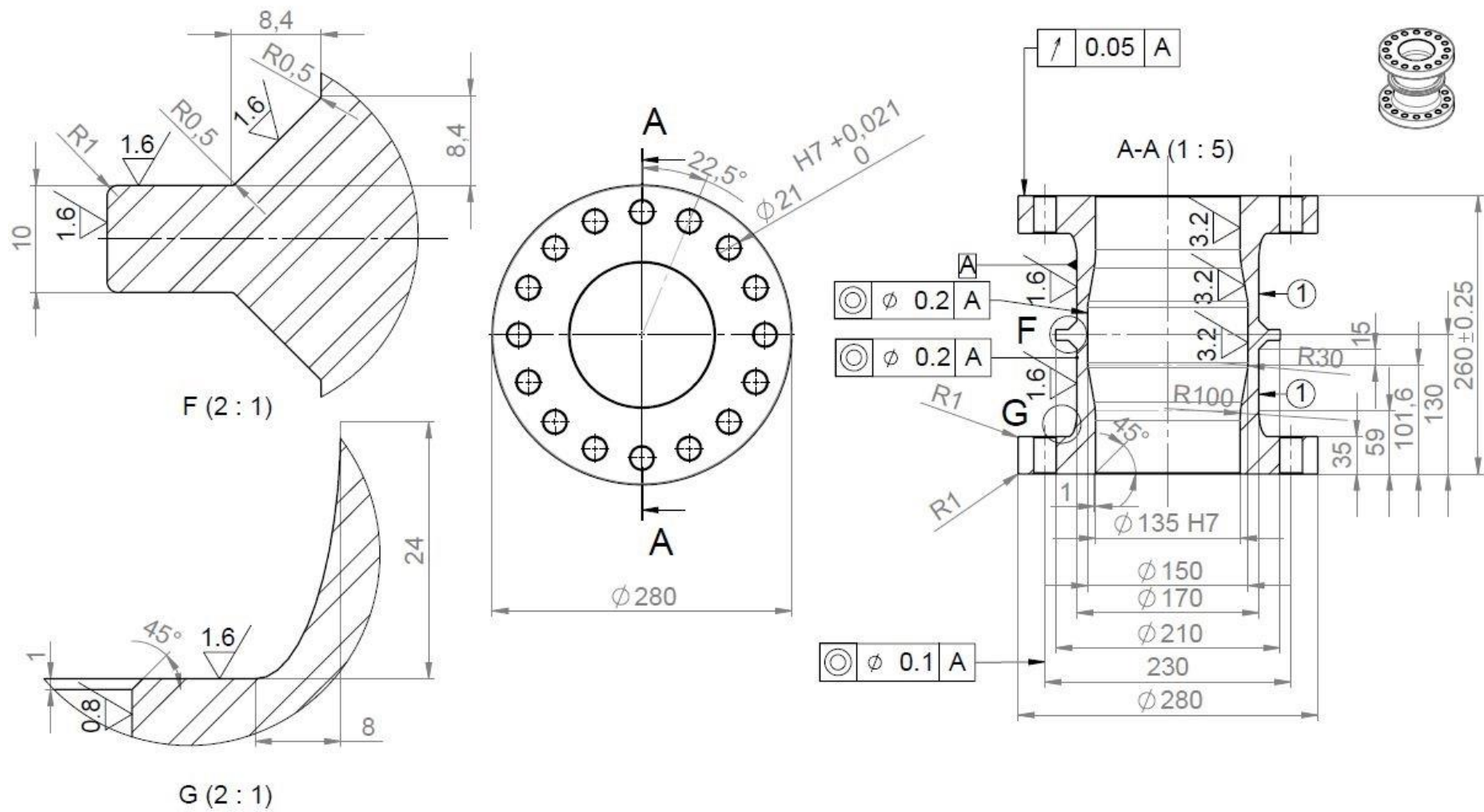
Figure 5.2: Technical drawing of the experimentally tested tubular specimen
