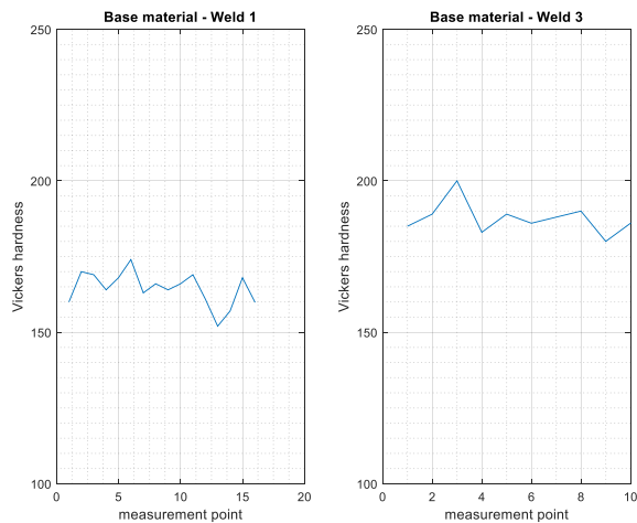
Figure 5.6: Hardness measurements in the base material of sample 1 (left) and sample 3 (right)
