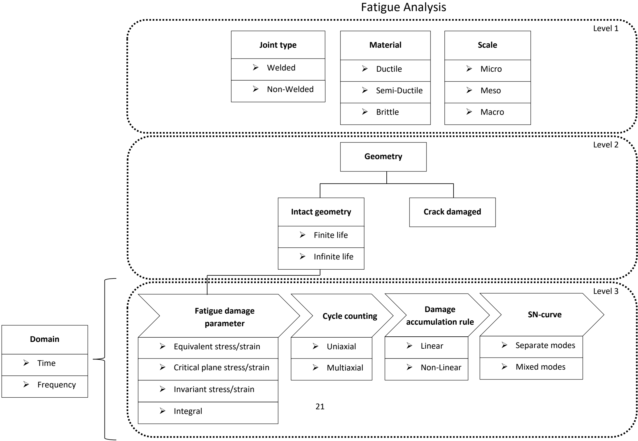
Figure 1.3: Schematic overview of the decision making process in the fatigue analysis of marine structures
