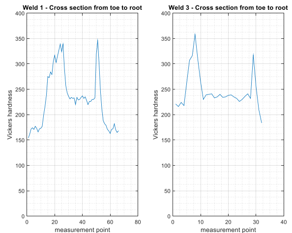
Figure 5.7: Hardness measurements in sample 1 (left) and sample 3 (right), through the weld from toe to root
