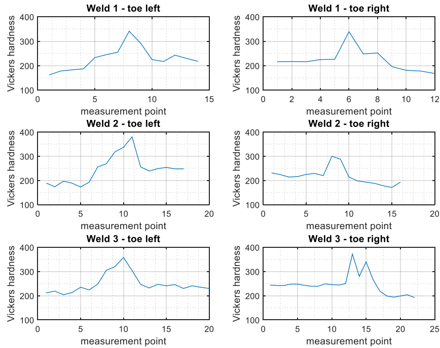
Figure 5.8: Hardness measurements in sample 1, 2 and 3 through the weld toe
