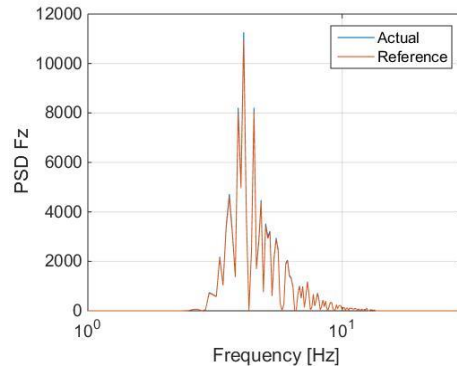
Figure 3.11: The power spectral density (PSD) distribution of random loading
