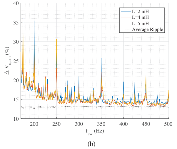
Fig. 4: Simulated maximum voltage ripple in submodule capacitors with f_{sw} for C_{sm}/N = 0.22 mF and for (a) varying N with L_{arm} = 5 mH (b) varying L_{arm} with N = 9 .
