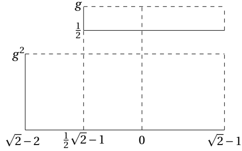
Figure 3.10: \Omega_{\sqrt{2}-1}
