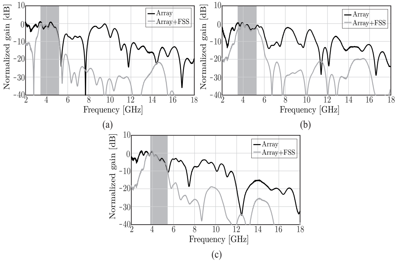
Figure 2.16: Measured active element gain normalized by the ideal directivity of the unit cell aperture, with and without the FSS for (a) broadside, (b) E - and (c) H -plane at 45^\circ .
