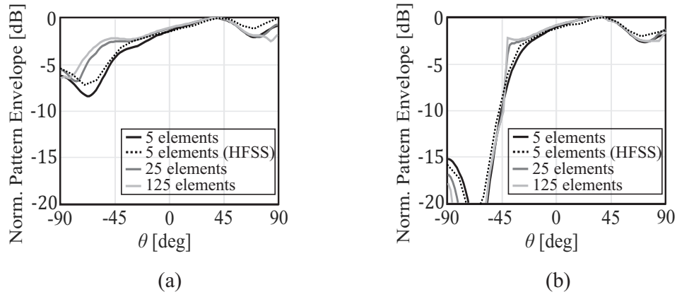
Figure 3.14: Pattern envelope as a function of the number of elements for a linear array of stacked dipoles in the presence of a backing reflector. The inclination angle is \alpha = 30^\circ and the distance between elements is (a) d_x = 0.5\lambda and (b) d_x = 0.6\lambda .
