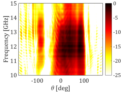
Figure 4.12: Color map of normalized active element pattern of element 5 at different frequencies.
