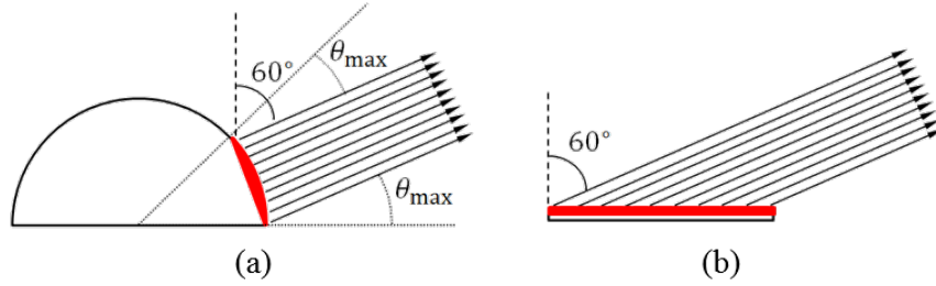
Figure 1.5: Maximum scan angle for (a) conformal and (b) planar array.
