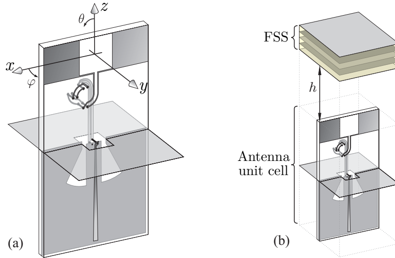
Figure 2.13: (a) Connected dipole unit cell and (b) 3D view of the MEFSS and the connected dipole array combined.
