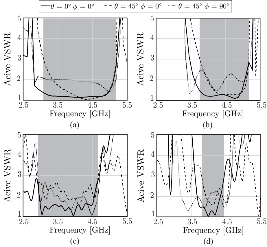
Figure 2.15: Simulated Active VSWR of (a) the array alone and (b) the dipole with the FSS, and measured Active VSWR of (c) the array and (d) in combination with the FSS.
