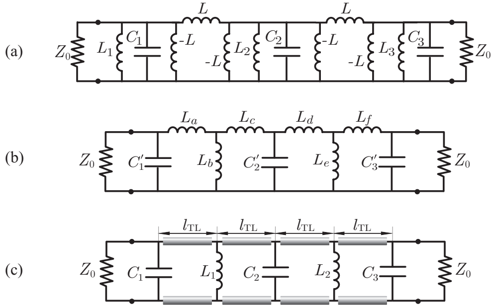
Figure 2.2: (a) Transformation of the admittance inverters shown in Fig. 2.1(c) into a Pi-network of inductances, (b) Pi-to-T transformation between inductances, and (c) final equivalent circuit where the series inductances are replaced by short transmission lines.
