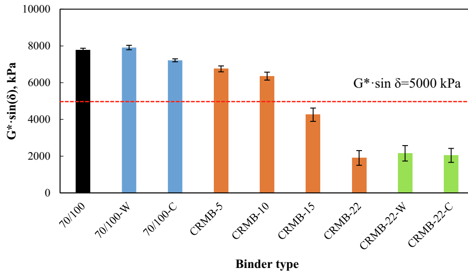
Fig. 5. Superpave fatigue parameters of different binders.
