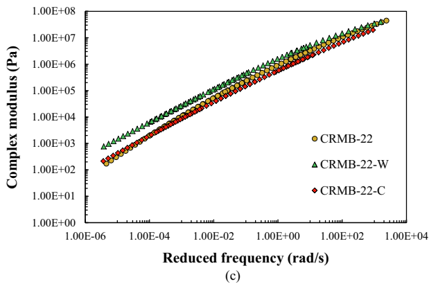
Fig. 10. Complex shear modulus master curves of binders at 20 °C: (a) CRMB with different CRM contents; (b) base bitumen with warm-mix additives; (c) CRMB with warm-mix additives.
