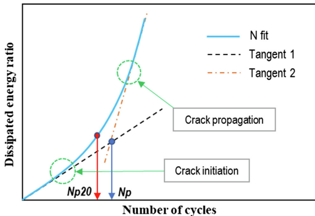
Fig. 4. Variation in the DER for a strain-controlled TS test.
