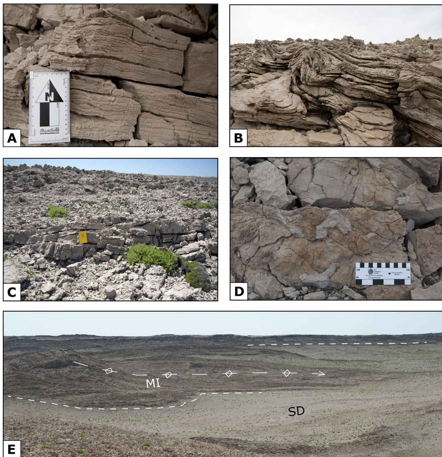
Figure 2 – Field pictures of the AdCP Milna and Sveti Duh Formations. (A) Detail of a stromatolite-rich interval. (B) Slumped laminated limestones. (C) Pinch-outs of channelized packstone-grainstone cross laminated interval within the Milna Formation. (D) The stained and burrowed surface at the interface between the Milna and Sveti Duh Formations. Plagues of light grey wackestone infill strata-parallel burrows. (E) Panoramic view of the sharp contact of the Sveti Duh Formation with the Milna Formation.
