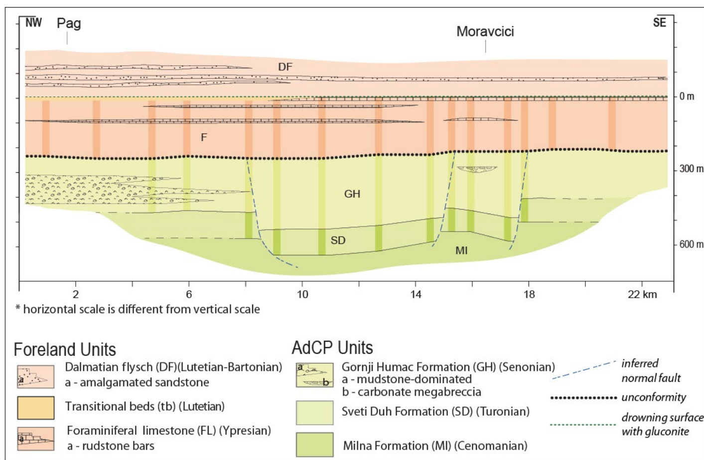
Figure 8 – Relations between faults and sedimentation. The thicknesses of the sedimentary formations as measured along the SW limb of the Pag anticline, restored to a horizontal top-foraminiferal limestone. Columns in darker colour are the projection of thicknesses measured on the map on a vertical section striking NW-SE. The variations in the facies associations is represented as well.
