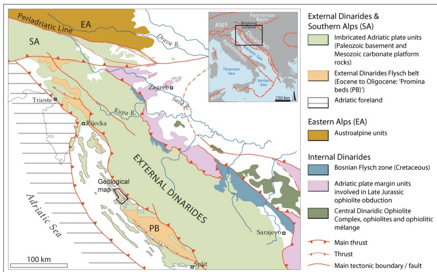
Figure 1 – Location of the map within a simplified regional scheme of the northern Dinarides (redrawn and simplified after Tomljenović et al., 2008; Ustaszewski et al., 2008; Korbar, 2009).
