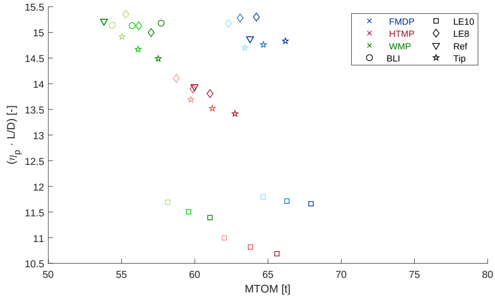
Fig. 16 Overview of (\eta_p \cdot L/D) vs MTOM for 10-30% \phi and high technology scenario for R = 1100\text{nmi} and M = 0.6 . Lighter color shades indicate lower \phi .
