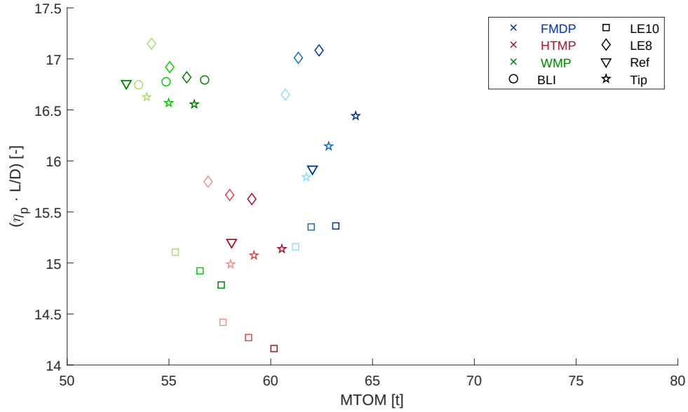
Fig. 20 Overview of (\eta_p \cdot L/D) vs MTOM for 10-30% \varphi and high technology scenario for R = 1100\text{nm} and M = 0.5 . Lighter color shades indicate lower \varphi .
