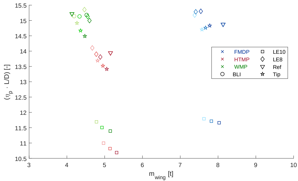
Fig. 21 Overview of (\eta_p \cdot L/D) vs wing mass for 10-30% \varphi and high technology scenario for R = 1100\text{nm} and M = 0.6 . Lighter color shades indicate lower \varphi .
