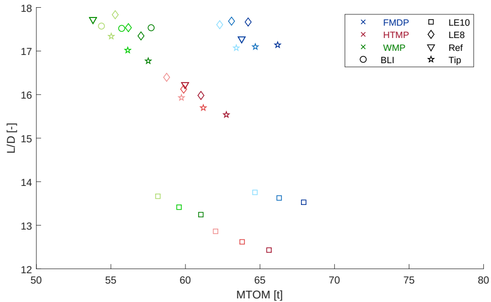
Fig. 17 Overview of L/D vs MTOM for 10-30% \phi and high technology scenario for R = 1100\text{nmi} and M = 0.6 . Lighter color shades indicate lower \phi .
