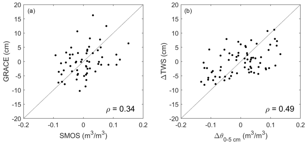
Figure 4. Scatter plots between the basin-averaged \Delta TWS and soil moisture anomaly ((a) GRACE Vs. SMOS, and (b) CABLE-estimated \Delta TWS and \Delta\theta_{0-5cm} ) of the Goulburn catchment. The correlation coefficient ( \rho ) is provided in each figure.
