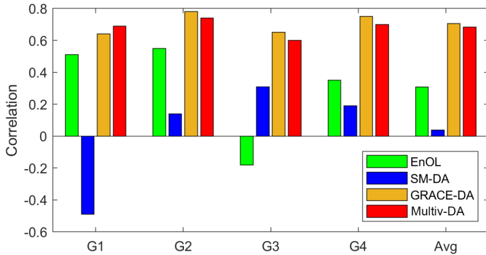
Figure 11. The correlation coefficients of the \Delta GWS estimates at (a) G1, (b) G2, (c) G3, and (d) G4 pixels computed from EnOL and different DA case studies. The averaged correlation values (Avg) of G1 – G4 are also shown.
