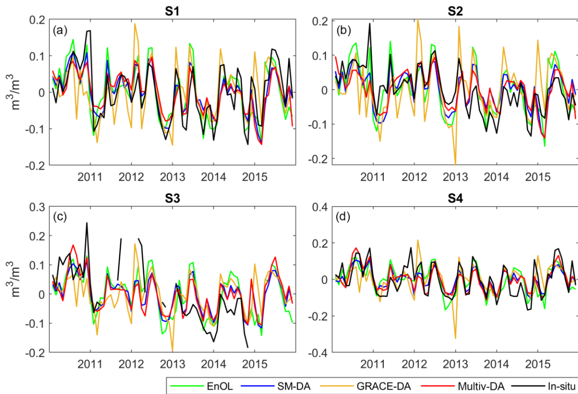
Figure 7. The monthly “0 – 5 cm” soil moisture variations estimated at S1 – S4 pixels computed from different DA approaches (SM DA, GRACE DA, and multivariate DA). The EnOL estimates and the in situ soil moisture data are also shown for comparison.
