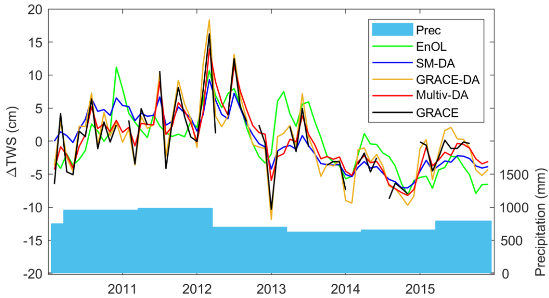
Figure 5. The monthly basin-averaged \Delta TWS computed from different DA approaches (SM DA, GRACE DA, and multivariate DA). The EnOL estimate, the GRACE observation, and the yearly precipitation accumulated between April and May are also shown for comparison.
