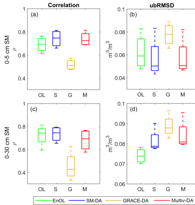
Figure 8. The correlation coefficients (a, c) and unbiased root mean square differences (ubRMSD; b, d) of the 0 – 5 cm soil moisture (top row) and 0 – 30 cm soil moisture (bottom row) computed from the estimate of different DA case studies at S1 – S4 (S: SM DA, G: GRACE DA, M: Multivariate DA). The statistical results of the EnOL (OL) are also shown.
