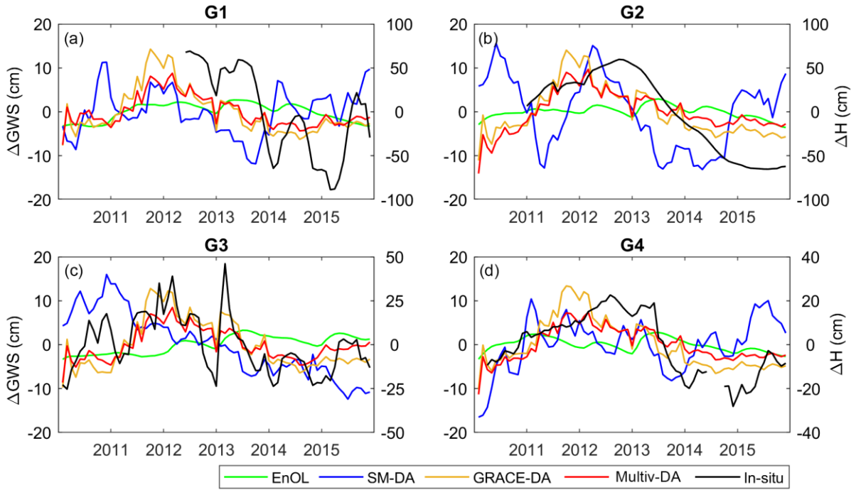
Figure 10. The monthly groundwater storage variations ( \Delta GWS ) at G1 – G4 pixels computed from different DA approaches (SM DA, GRACE DA, and multivariate DA). The EnOL estimates and the in situ groundwater level variations ( \Delta H ) are also shown for comparison.
