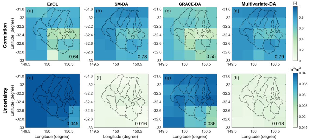
Figure 3. The correlation coefficients (top row) and uncertainty (ensemble spread, bottom row) of the 0 – 5 soil moisture estimates computed between the SMOS data and different DA case studies. The averaged correlation and error values of the Goulburn catchment are given in each figure.
