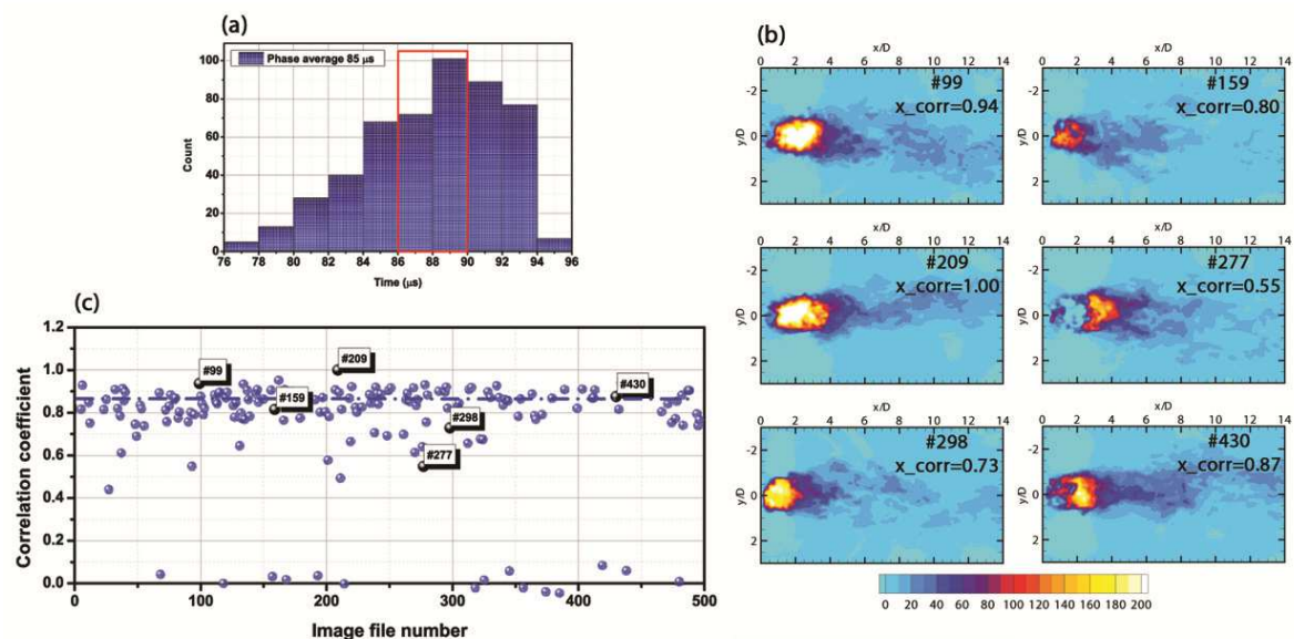
Figure 13: (a) Distribution of real time delays, (b) six instantaneous flow fields at a same real time delay of 86 \mu s, and (c) spatial correlation coefficient in the series of 500 instantaneous. All figures correspond to an acquisition delay imposed at 85 \mu s
