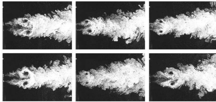
Figure 12: Illustration of the seeded flow at a constant time delay of 125 \mu s.
