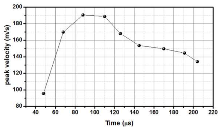
Figure 16: Peak velocity value at different time delays
