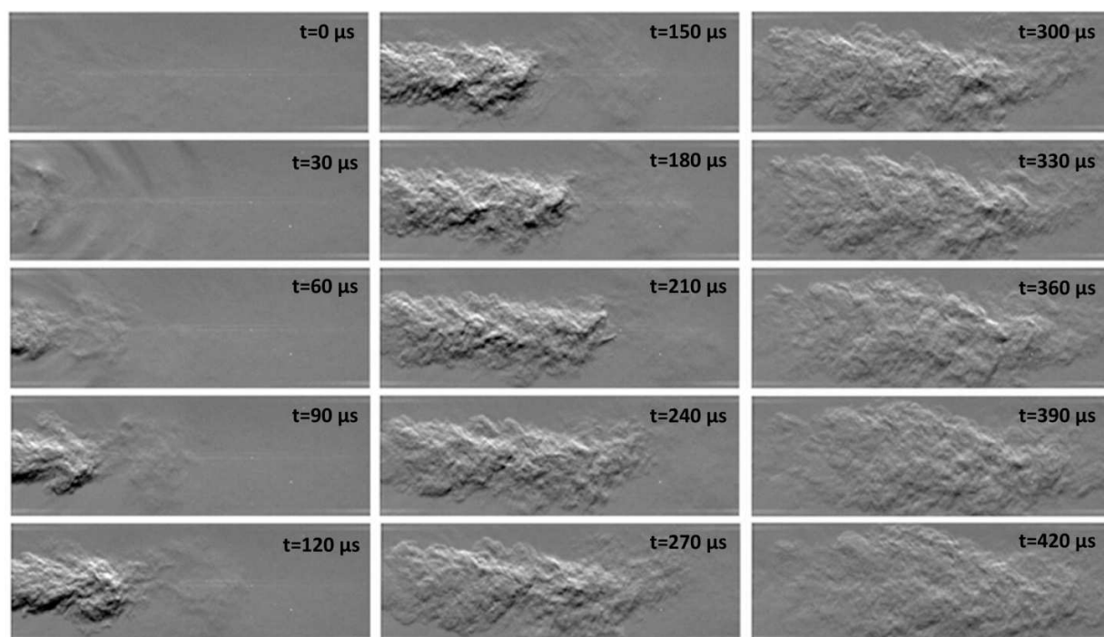
Figure 9: Time evolution of the 3-mm jet perturbed by a single arc discharge depositing 48 mJ at the internal jet throat. Exposure time of 1 \mu s.
