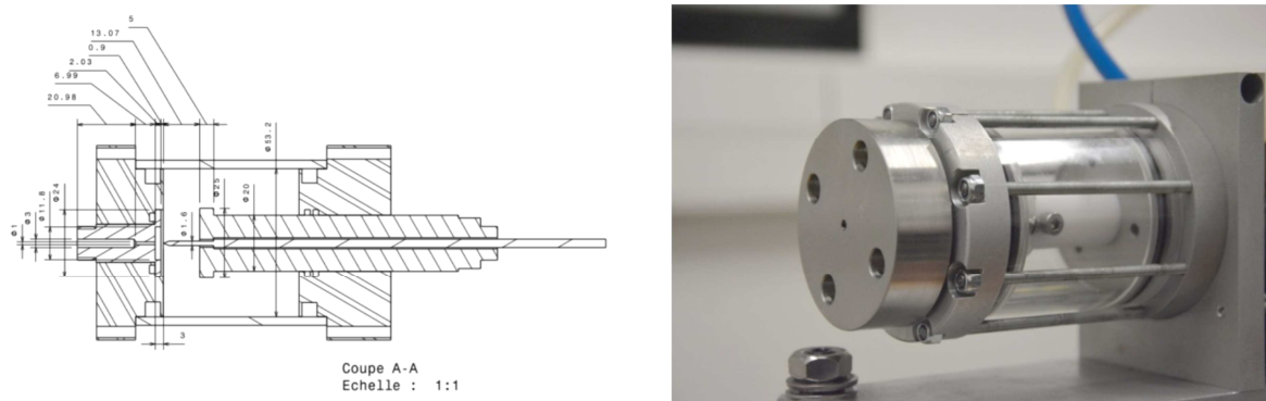
Figure 2: Technical drawing of the initial model and image of the plasma-assisted jet in subsonic (long neck extension) configurations
