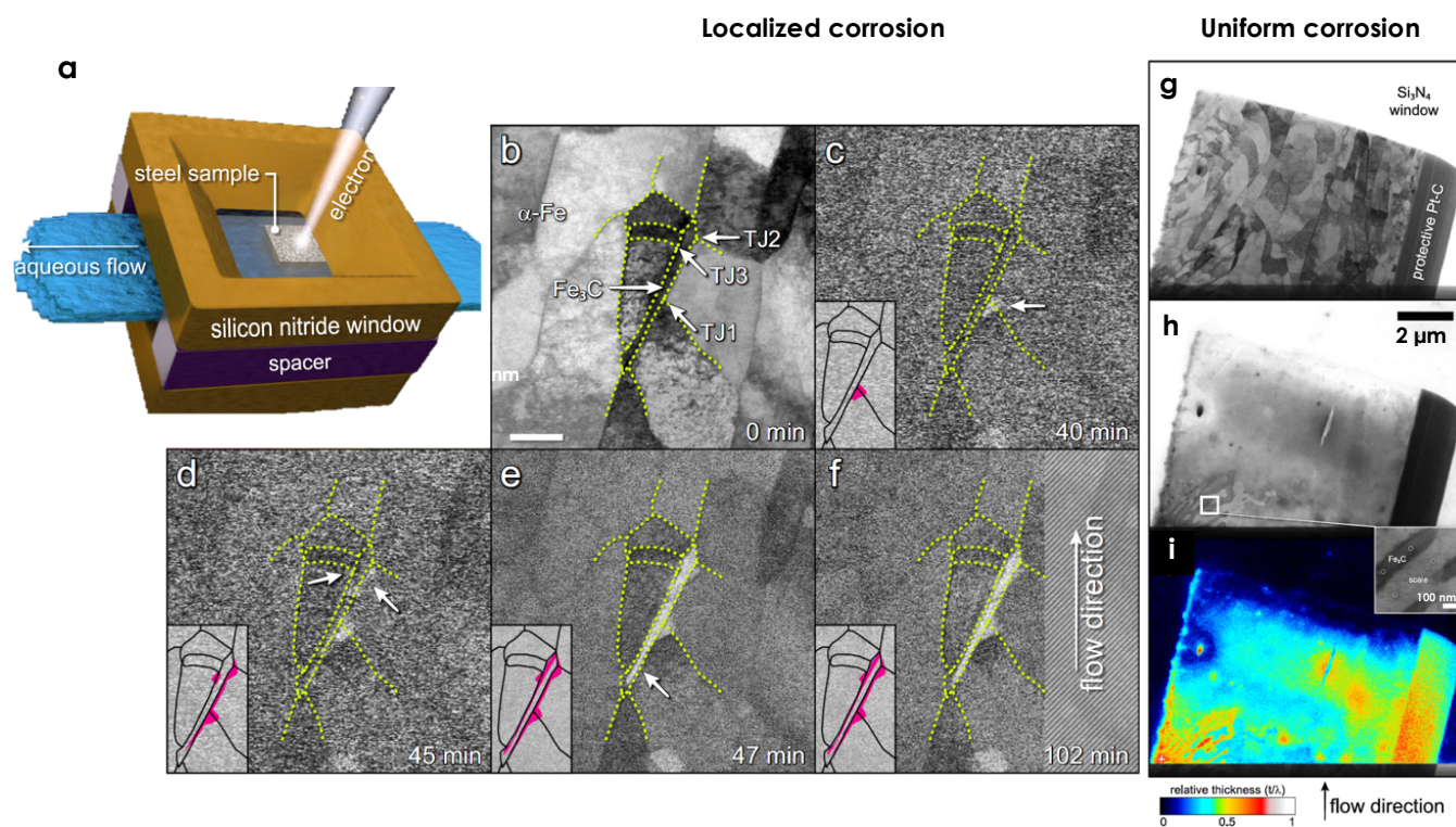
Fig. 10, (a) Schematic of the liquid cell loaded with a 1018 steel lamella. (b) Bright field STEM image of a region that was microstructurally and chemically characterized before exposure to 2.78 \mu\text{M Na}_2\text{SO}_4 solution. A cementite grain inclusion fully confined by a ferrite matrix and different triple junctions TJ1, TJ2, and TJ3 indicated by white arrows. (c–f) Time-resolved bright field STEM images of the region during exposure to the flowing solution. Having initiated at TJ1, localized corrosion took place in the 1018 steel sample at the phase boundary between ferrite and cementite. (g–i) Concurrent occurrence of uniform corrosion revealed by bright field STEM micrograph of the lamella (g) before, and (h) after 1025 min exposure. (i) Energy filtered TEM to relatively map the thickness of the corroded specimen. Reproduced from Hayden et al., 115 with permission from Springer Nature. The images were originally published as parts of three distinct figures.
