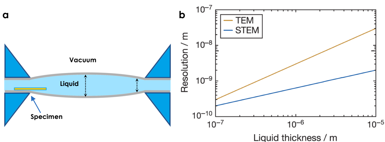
Fig. 5, (a) Schematic cross-section of a liquid cell placed in vacuum, showing bulging of the membranes which gives rise to a location-dependent liquid thickness. Therefore, TEM lamellae should be placed close to the edge of the window where bulging is minimum. (b) Maximum resolution versus thickness of water in TEM and STEM. The resolution is theoretically calculated for typical instrument parameters at 200 keV to image Au nanoparticles at the bottom of a layer of water for TEM, and at the top of the layer for STEM. Adapted from De Jonge and Ross 25 with permission from Springer Nature.
