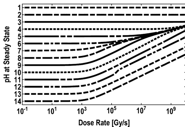
Fig. 6, Influence of initial pH prior to irradiation and dose rate on steady state pH of the radiated region. The values are theoretically calculated for de-aerated water. The gray per second (Gy/s) is defined as the absorption of one joule per kilogram of matter per unit time. Reprinted from Schneider et al., 82 with permission from American Chemical Society.
