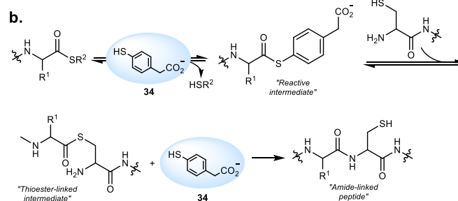
Figure 4: Proposed catalytic mechanisms: a. Aniline ( 32 ) -catalysed hydrazone ( X=NH )/ oxime ( X=O ) formation. b. Aryl thiol-catalysed native chemical ligation (NCL).
