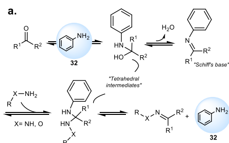
Figure 4: Proposed catalytic mechanisms: a. Aniline ( 32 ) -catalysed hydrazone ( X=NH )/ oxime ( X=O ) formation. b. Aryl thiol-catalysed native chemical ligation (NCL).
