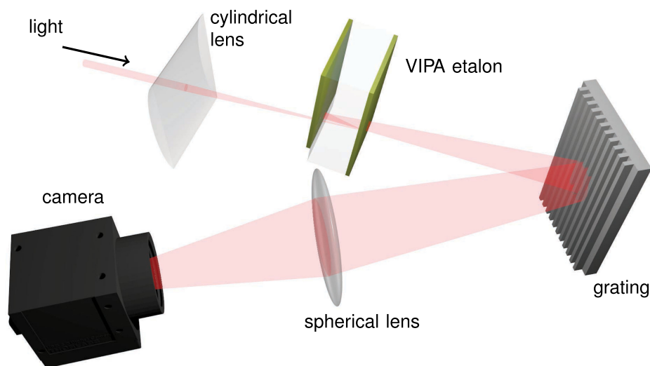
Fig. 3. A schematic of the VIPA spectrometer. Light is focused using a cylindrical lens on the VIPA etalon which then disperses the light spectrally in the y-direction. A grating is used as a post-disperser in the x-direction to separate the different orders. The angularly dispersed frequency information is then converted to position information on a camera.
