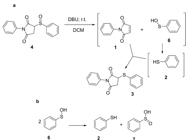
Figure 3. (a) Proposed elimination of sulfoxide 4. (b) Proposed disproportionation of sulfenic acid 6 to give thiophenol 2 and sulfonic acid 7. The compounds in brackets (maleimide 1, sulfenic acid 6 and thiol 2) indicate that they could be the intermediates which were not detected during characterization).
