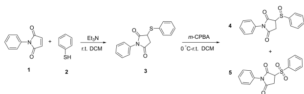
Figure 2. The conjugate addition of thiophenol 2 with N -phenylmaleimide 1 and the subsequent oxidation of 3 by m -CPBA.
