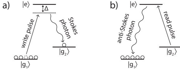
Figure A.1: Schematic of the processes used in the DLCZ scheme. a) Write process based on spontaneous Raman scattering under off-resonant driving of the |g_1\rangle - |e\rangle transition. b) Highly efficient readout of the memory state by resonantly driving on the |g_2\rangle - |e\rangle transition.
