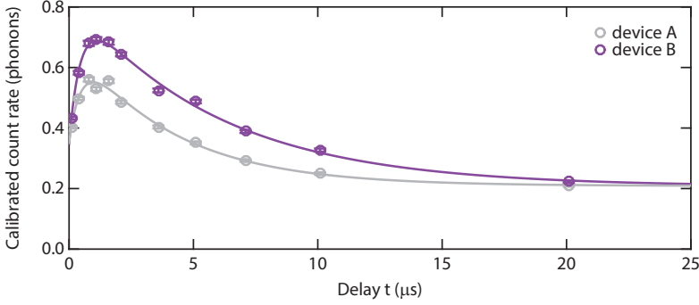
Figure 4.7: Pump-probe experiment. The experiment reveals the response of the devices mechanical modes to the initial optical pump. See text for details. Error bars are s.d.
