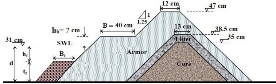
Fig. 4. Configuration of the berm breakwater model.
