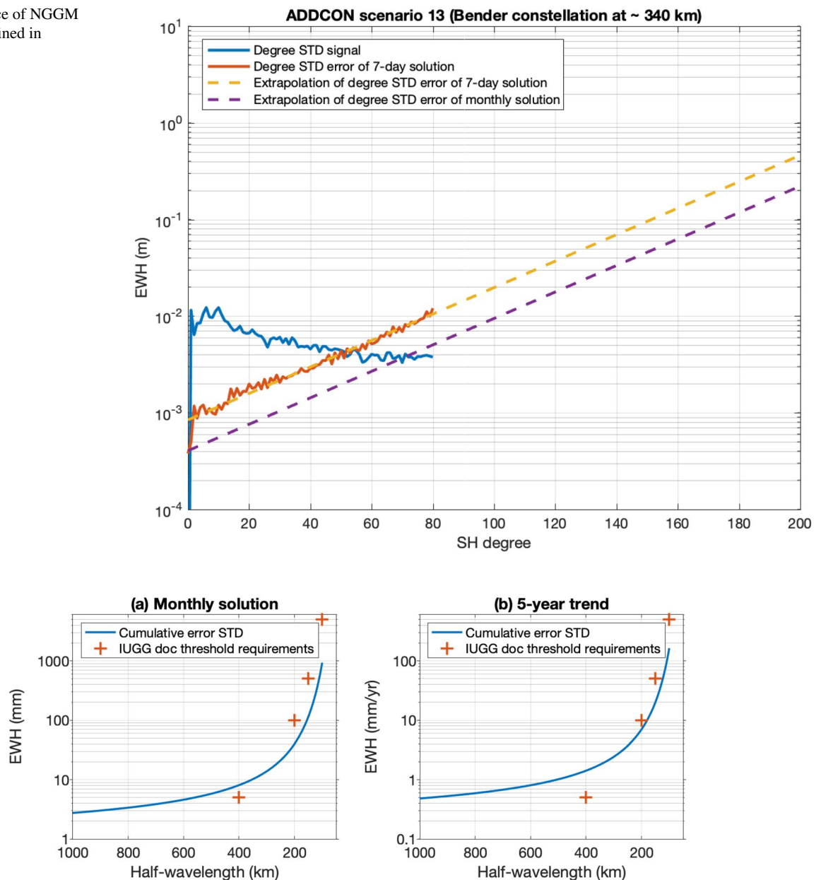
Fig. 5 Square-root of cumulative degree variance of NGGM scenario 13 as defined in Table 2. The left panel shows the extrapolation from weekly to monthly gravity field solutions (blue curve) and the threshold requirements for the monthly gravity field solutions (red crosses).
