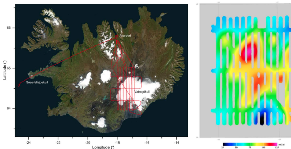
Fig. 8 Flight paths over Iceland and gravity measurements (left) and gravity measurements along the flight grid (right). Courtesy: Y Bidet, ONERA
