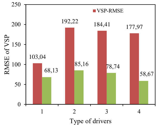
Fig. 10. Result of VSP-RMSE after calibration of SDX
