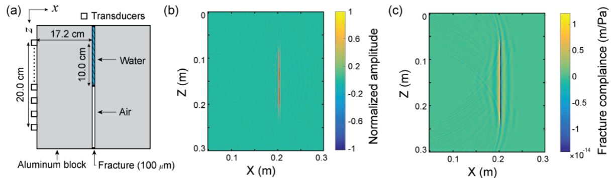
Figure 1 (a) Configurations of laboratory experiments. (b) Imaging result with conventional reverse-time migration. (c) Imaging result with the proposed least-squares migration.
