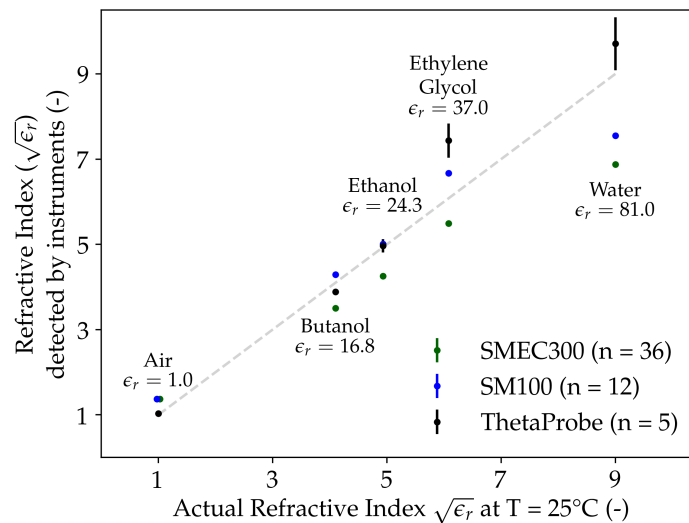
Figure 3. Response of the capacitive soil moisture sensors (SMEC300 and SM100) and secondary standard (impedance-based ThetaProbe) to fluids of known \epsilon_r at 25 °C. The X- and Y-axis depict the actual and measured refractive indices ( \sqrt{\epsilon_r} ), respectively. Although the ThetaProbe measures \sqrt{\epsilon_r} directly, the VWC values of SM100 and SMEC300 were converted to the corresponding \sqrt{\epsilon_r} values based on the literature [10]. n is the total number of measurements in the experiment of a fluid, and the error bar shows the mean and standard error of the estimated values.
