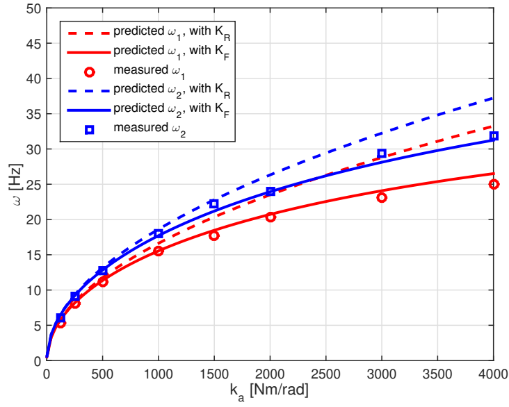
Figure 6: The predicted values for the two lowest natural frequencies, using either the rigid-body stiffness model or the flexible-body stiffness model, as well as the measured natural frequencies as a function of actuator stiffness values.
