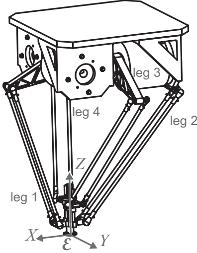
Figure 1: The Heli4 manipulator is modeled as a 4-RRRIR robot. All twists, wrenches and matrices are expressed in the Cartesian end-effector reference frame \mathcal{E} .
