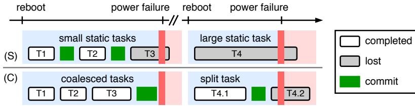
Figure 4.1: Task coalescing reduces commit overhead (left), while task splitting enables termination of large tasks (right). S: static legacy task-based runtime, C: Coala (this work).
