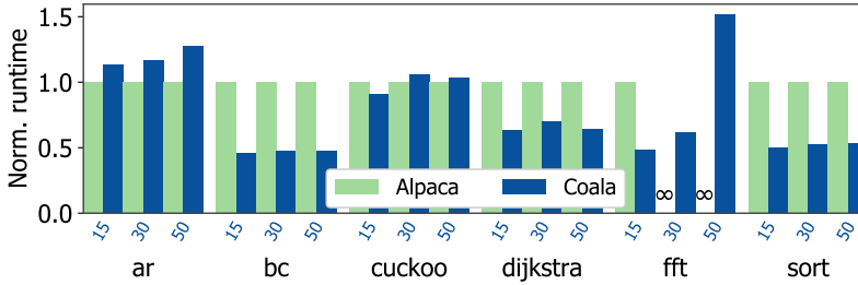
Figure 4.10: Coala's execution time normalized to Alpaca's, for three distances from the energy source (15, 30 and 50 cm).
