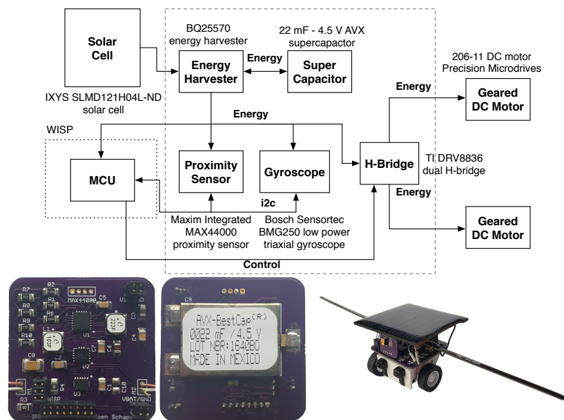
Figure 3.7: Battery-less small autonomous robot: top figure—block diagram; bottom left—robot PCB design (front side): harvester (U1), gyroscope (U2) and H-bridge (U3); bottom center—robot PCB design (back side): super-capacitor, bottom right—complete robot.
