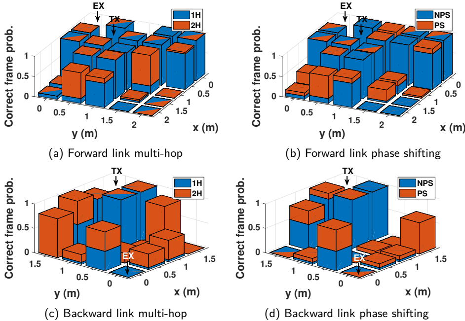
Figure 6.10: Backscatter T2T network phase cancellation experiment. EX and TX mark the positions of the exciter and transmitter, respectively. ( N ) PS : (no) phase shifting. Figure 6.10a and 6.10b: forward link. Both methods yield comparable results. Figure 6.10c and 6.10d: backward link. Multi-hop is superior in network coverage. Note: 1H and NPS is the same case.
