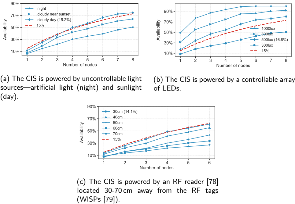
Figure 5.11: The Coalesced Intermittent Sensor’s availability for differed numbers of intermittent nodes and energy sources. The modeled availability—represented by the dashed lines when the average node duty cycle is 15%—approximates the measured availability with high accuracy.
