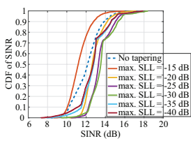
Fig. 4. Impact of max. SLL with amplitude tapering on the SINR performance for min. inter-user spacing of 1.2\lambda/D .
