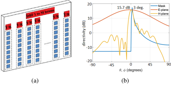
Fig. 1. 5G cosecant subarray beamforming [10], (a) uniform linear array of subarrays (b) cosecant-square power distribution in elevation.
