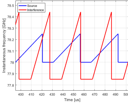
(a) Instantaneous frequency in FMCW radars.
