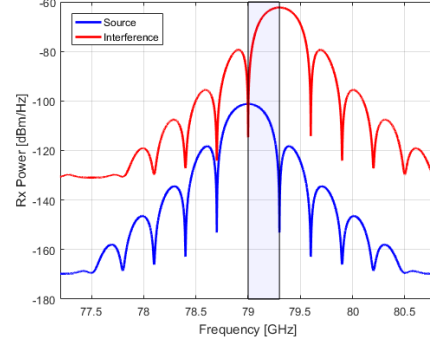
(b) Time-invariant, sinc-shaped spectrum of single-carrier binary PMCW waveforms.
