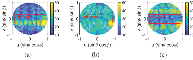
Fig. 8. Far E -field patterns (in dBV/m) of the 8 \times 8 patch array in Case-6 for a beam scanned toward the 5G cell sector edge u_s = \sin(\pi/3) , v_s = -\sin(\pi/12) for (a) progressive phases, (b) phases optimized for minimum SLL everywhere in the visible region, and (c) phases optimized for minimum SLL in the sector.
