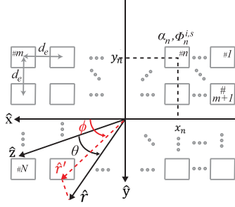
Fig. 1. Schematic of a uniform planar array of N patch antennas. \theta is the elevation angle defined as the angle between the observation direction \hat{r} and \hat{z} . The unit vector \hat{r}' is the projection of \hat{r} onto the \hat{x}\hat{y} plane. \phi is the azimuth angle defined as the angle between \hat{r}' and \hat{x} .
