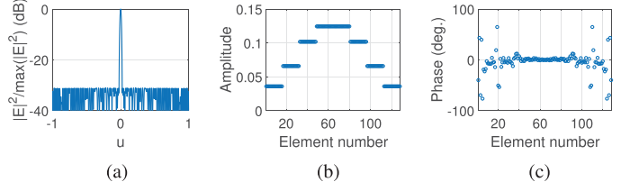
Fig. 4. Results of Case-3 for N = 128 , Q = 8 . (a) Normalized AF. (b) Even-symmetric element amplitudes. (c) Even-symmetric element phases.
