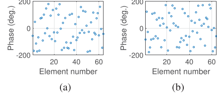
Fig. 9. Element phases at iteration number 25 with \mu = \pi/3 in Case-6 with optimization for minimum SLL (a) everywhere in the visible region and (b) only in the sector.
