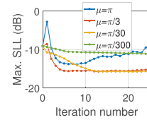
Fig. 10. Maximum SLL trend with \mu for optimization everywhere in the visible region.
