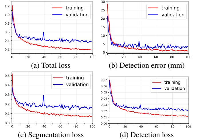
Figure 5: Learning curves for the chosen hyperparameter setting.
