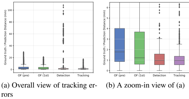
Figure 6: Tracking errors for the 4 methods on all test images.
