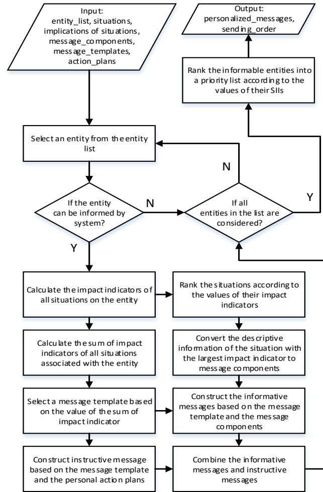
Fig. 3. The workflow implemented for constructing personalized messages
