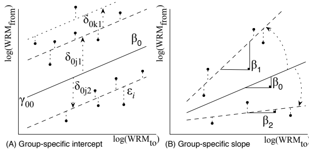
Fig. 9. Visual representation of group-specific intercept and slope. In figure A, the intercept is allowed to vary but regression lines stay parallel; the total group-specific intercept is \gamma_{00} + \delta_{0j} + \delta_{0k} . In figure B, slopes are allowed to vary, leading to a different \beta per group.
