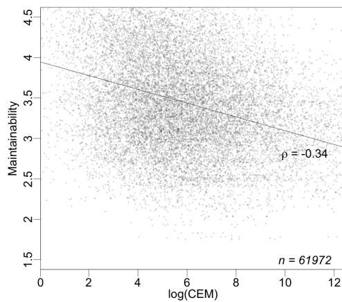
Figure 4. The correlation between the SIG Maintainability rating and log(CEM). Logarithmic transformations have been applied to demonstrate the relationships more clearly. This does not affect the strength of the correlation.
