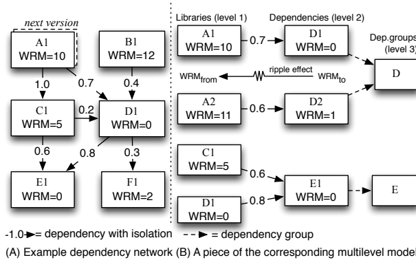
Fig. 7. An example of libraries and their dependencies. On the right side, the corresponding multilevel representation of the left side is shown. Not all nodes and relationships from panel A are included in panel B.
