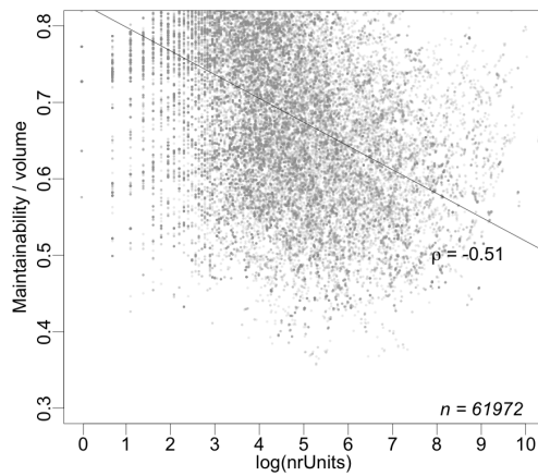
Figure 3. The correlation between the SIG Maintainability rating and system size as measured in number of units. Logarithmic transformations have been applied to demonstrate the relationships more clearly. This does not affect the strength of the correlation.
