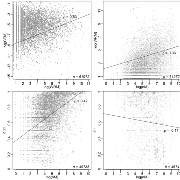
Fig. 3. Scatterplots and Spearman rank correlations between, CEM, WRM, number of methods (nM) and average incoming (inI) and outgoing isolation rating (outI). The axis limits have been adjusted and logarithmic transformations have been applied to demonstrate the relationships more clearly.
