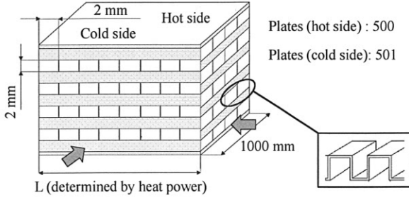
FIGURE 10. Geometry and configuration of the printed circuit regenerator of the \text{scCO}_2 waste heat recovery unit.
