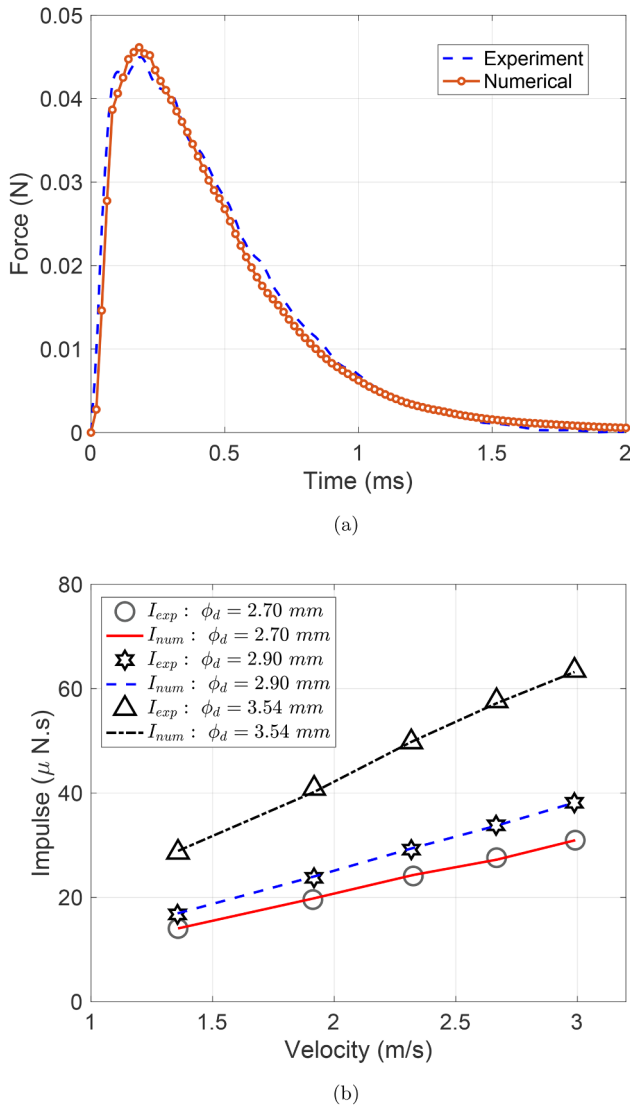
Fig. 13. (a) Comparison of contact forces for \phi_d = 2.7 mm and V_d = 2.67 m/s (b) Comparison of impulses for various cases of droplet size and impact velocity.
