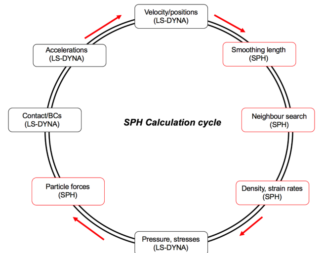
Fig. 6. Calculation cycle of SPH method in LS-DYNA [38].
