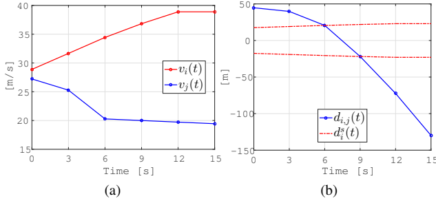
Fig. 3: Example of longitudinal collision: (a) Velocity profiles. (b) Relative and safety distances.
