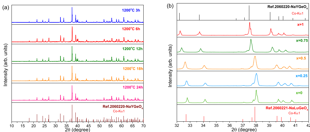
Figure 2. XRD patterns for (a) \text{NaYGeO}_4:0.01\text{Bi}^{3+} synthesized at 1200 °C during 3–24 h and (b) \text{NaLu}_{1-x}\text{Y}_x\text{GeO}_4:0.01\text{Bi}^{3+}, 0.001\text{Eu}^{3+} ( x = 0-1 ) solid solutions.
