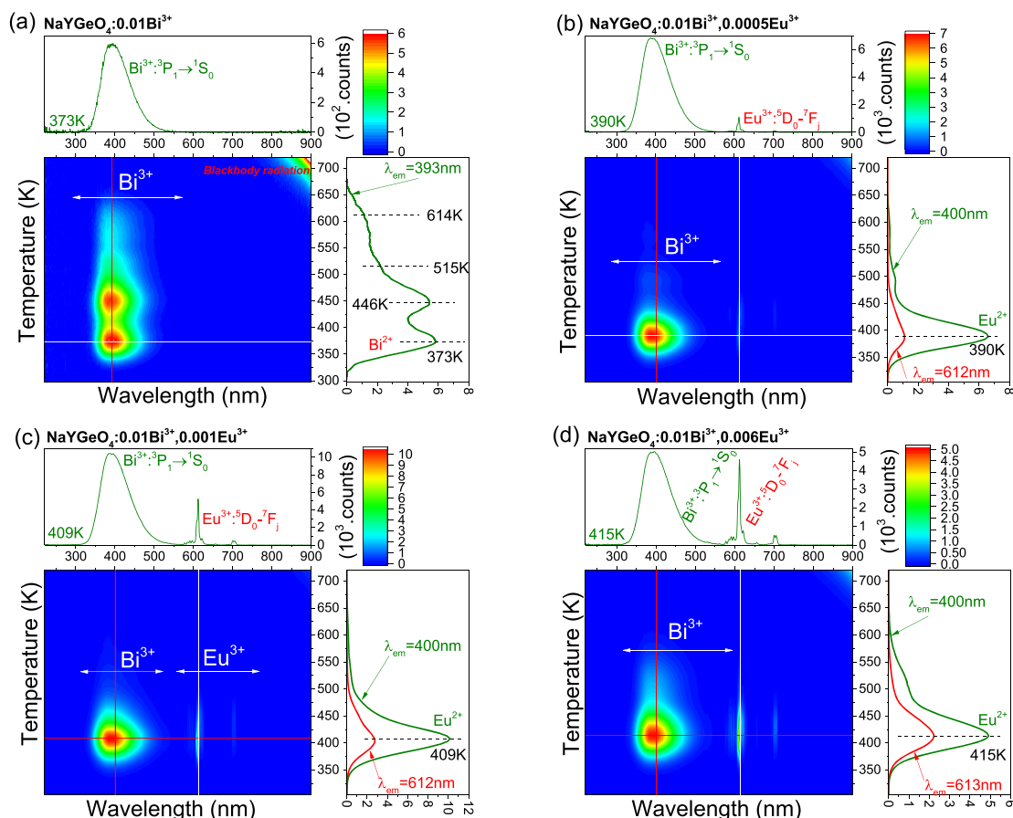
Figure 6. Thermoluminescence emission (TLEM) spectra for (a) NaYGeO 4 :0.01Bi 3+ synthesized at 1200 °C during 24 h, (b) NaYGeO 4 :0.01Bi 3+ , 0.0005Eu 3+ , (c) NaYGeO 4 :0.01Bi 3+ , 0.001Eu 3+ , and (d) NaYGeO 4 :0.01Bi 3+ , 0.006Eu 3+ at \beta = 1 K/s after \gamma -ray irradiation.
