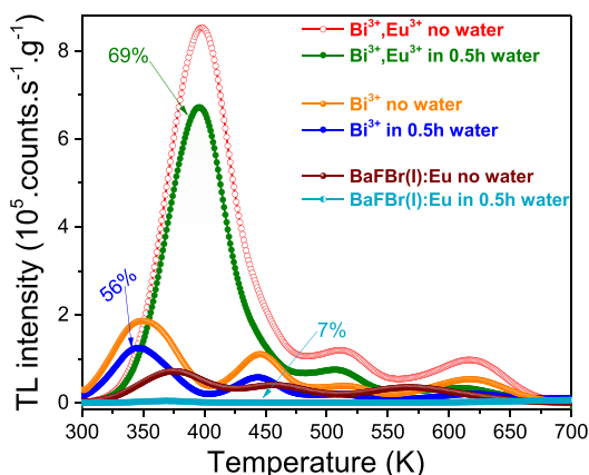
Figure 10. TL glow curves at \beta = 1 K/s for \text{NaYGeO}_4:0.01\text{Bi}^{3+} , \text{NaYGeO}_4:0.01\text{Bi}^{3+},0.001\text{Eu}^{3+} , and \text{BaFBr(I):Eu} after exposure to water after \beta -irradiation.
