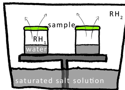
Fig. 4. Schematic of wet cup setup: The samples (green) are glued to the top of a water containing vial. The difference in RH between the inside of the vial and the RH in the desiccator acts as driving force for moisture permeation through the sample. The weight of the vials is measured in regular intervals to monitor the amount of water that passed through the samples. (For interpretation of the references to colour in this figure legend, the reader is referred to the Web version of this article.)
