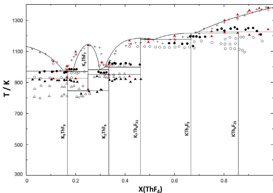
Fig. 11. Optimized KF-ThF 4 phase diagram superimposed against experimental points by Asker et al. (▲, +, ●) [9], Emelyanov and Evstyukhin (△, ●) [8], and this study (▲, liquidus onset ▽, red). (For interpretation of the references to colour in this figure legend, the reader is referred to the web version of this article.)
