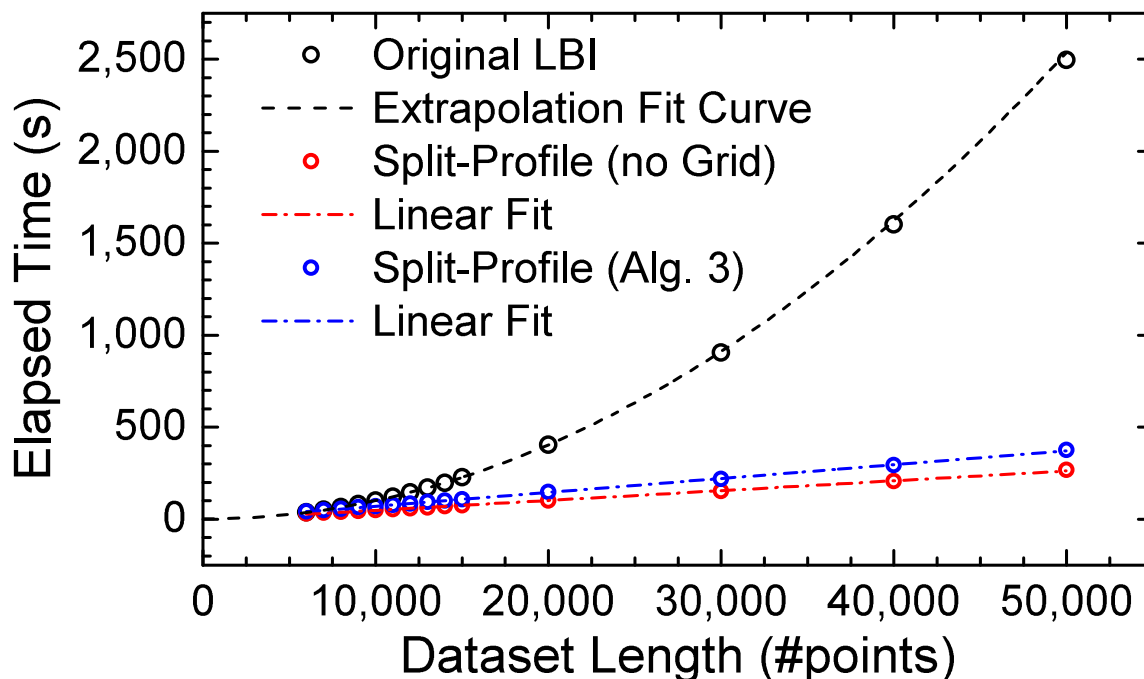
Figure 5. Final timing comparison between the original LBI and the corresponding split-profile LBI; two versions of the latter, with and without the \lambda -grid, are depicted. For shorter dataset lengths, the effect of the split-profile methodology is rather negligible since the original length is comparable to the individual split-profile length; however, as the dataset length increases above 20,000 points, a very clear distinction can be observed between the total elapsed times of the variants of the analysis algorithm.
