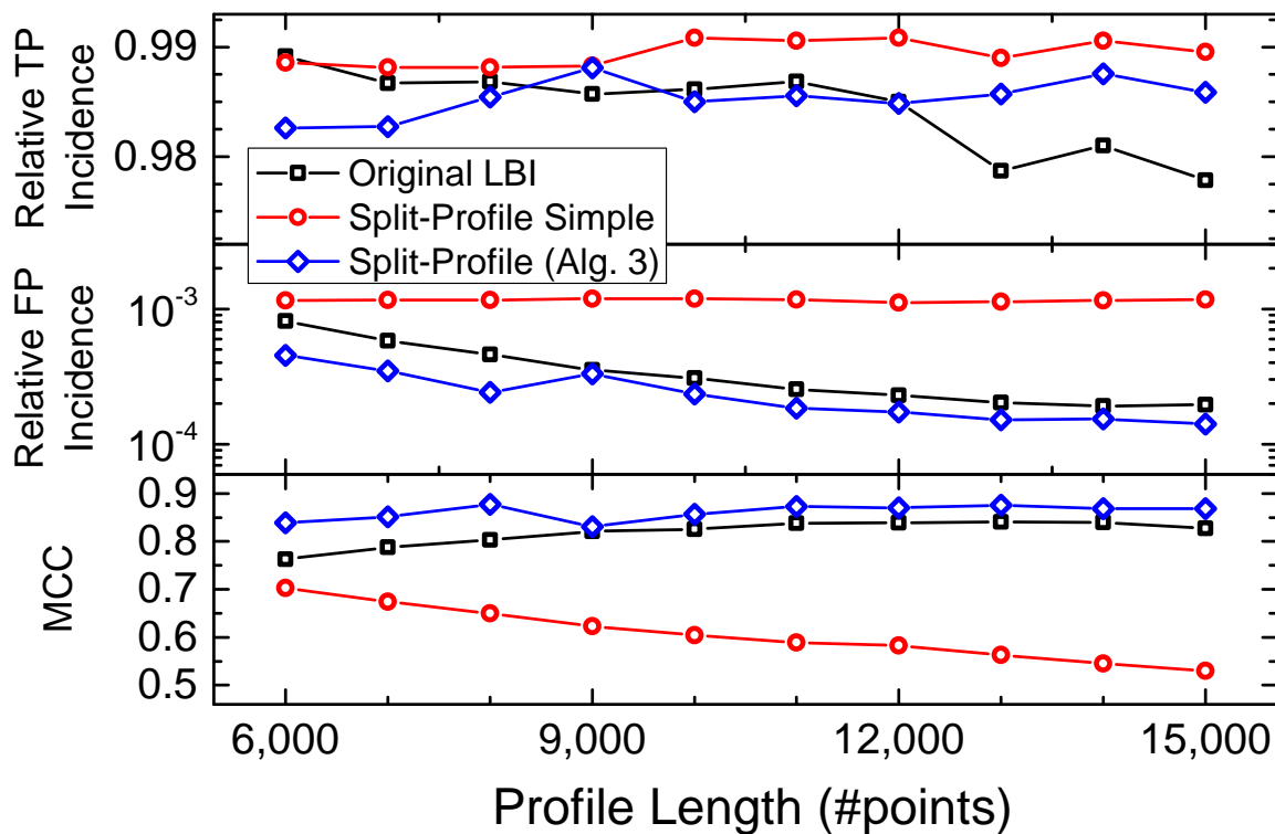
Figure 3. Performance comparison between three different versions of the analysis algorithm. Even though the differences of TPs and TFs might not seem extremely drastic for the split-profile simple, the broader characterization enabled by the MCC makes it clear that there is a deep performance drop if \lambda is not correctly chosen.
