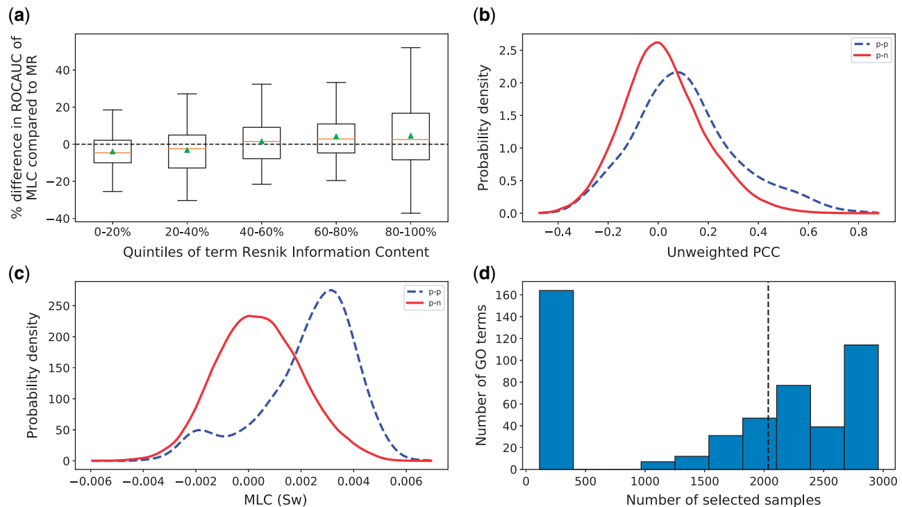
Fig. 2. (a) Percent increase in ROCAUC of MLC ( S_w ) with respect to MR as a function of Resnik IC. For each set of terms in each quintile of IC, the corresponding box includes the two middle quartiles of the percent increase for these terms. An orange line denotes the median and a green triangle the mean. The error bars extend to 1.5 times the range of the two middle quartiles. Note, that the 0–20% quintile corresponds to the 20% least specific terms and the 80–100% quintile to the 20% most specific ones. (b–c) Distributions of co-expressions for genes annotated with term GO: 1903047. In dashed blue lines, the co-expression values between a test and a training gene that both are annotated with that term. In solid red lines, the co-expression between test genes annotated with that GO term and training genes that are not. Co-expression is measured as the PCC (b) and the S_w trained by MLC (c). The x-axis shows the co-expression values and the y-axis the probability density estimated with Gaussian kernels. Note that the PCC and S_w have different ranges due to the weight optimization. (d) Histogram of the number of samples that were selected for each GO term. The x-axis corresponds to the number of selected samples and the y-axis to how many GO-term-specific similarity functions selected that many samples. The dashed line denotes the median number of non-zero weights
