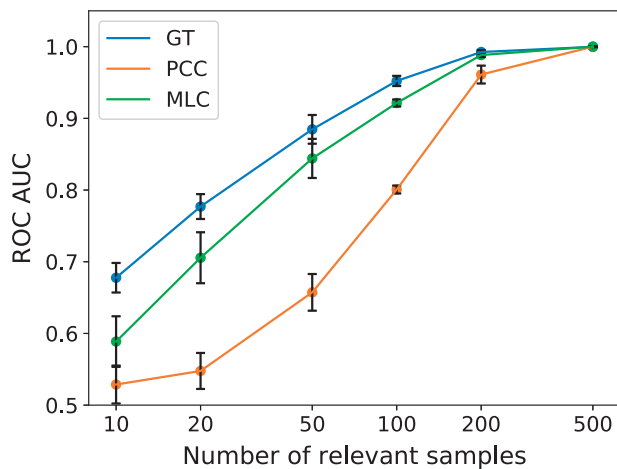
Fig. 3. ROCAUC (y axis) on simulated data as a function of the number of relevant samples (x axis on log scale) for MLC (green), PCC (orange) and the PCC using only the GT samples (blue). The error bars denote the SD over five repetitions
