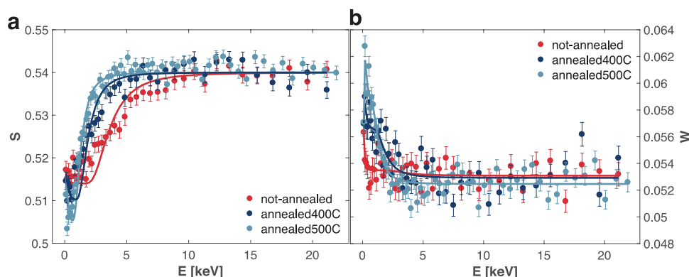
Figure 3. Positron Doppler broadening. a) S -parameter and b) W -parameter depth profiles of papain/titania nonalayers before and after thermal annealing at 400 and 500 °C for 4 h. Dashed lines are fit curves to a single layer and substrate model obtained using VEPFIT analysis (see Table 1).
