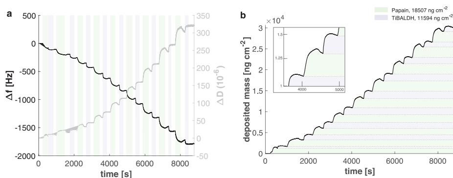
Figure 1. a) QCM-D measurement of the deposition of a papain/titania 9-layer. Green regions indicate immersion using 1 \times 10^{-3} M papain in 100 \times 10^{-3} M MOPS pH 7.0, blue regions indicate immersion using 20 \times 10^{-3} M TiBALDH, and the white regions stand for washes with distilled deionized water. b) Mass deposition extracted with QSense Dfind Composite Sauerbrey. [15]
