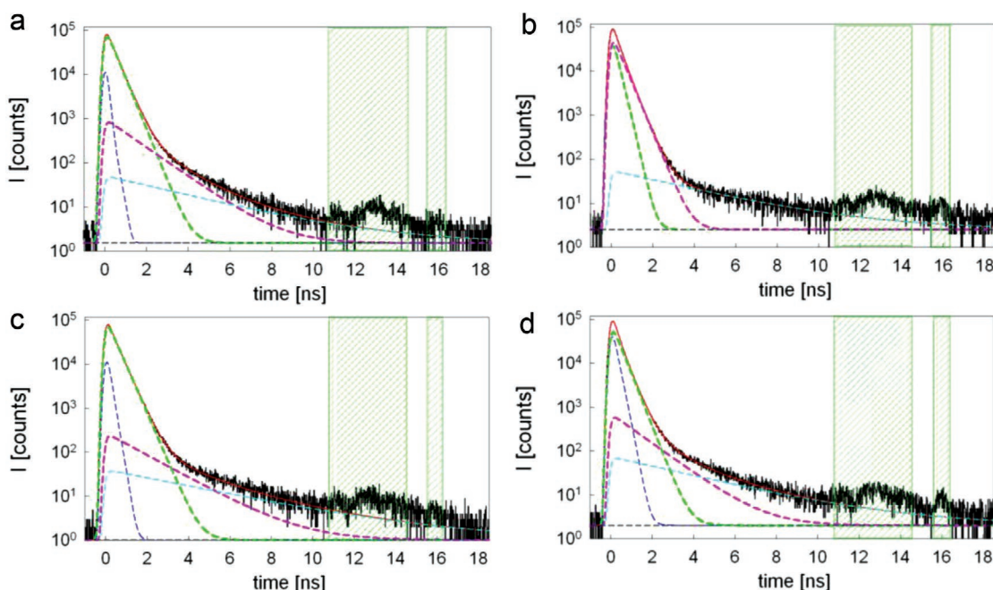
Figure 8. PALS spectra at 1 keV and fits obtained using POSWIN of a) papain/titania nonalayer, b) annealed (450 °C, 4 h) papain/titania nonalayer, c) TiO 2 reference sample fabricated using EBPVD, and d) ITO layer on glass substrate. The regions between 10.8 and 14.5 ns as well as 15.6–16.2 ns have been excluded from fitting, due to the presence of spurious peaks of annihilation by backscattered positrons.
