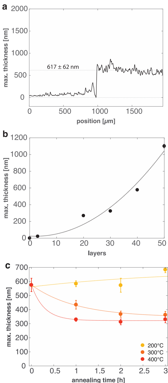
Figure 2. a) Profilometry thickness measurement of as-deposited papain/titania nonalayer. b) Thickness of papain/titania layers as a function of number of deposited layers using 10 \times 10^{-6} M papain in 20 \times 10^{-3} M MOPS pH 7.0, determined from profilometry. c) Thickness of papain/titania nonalayers deduced from profilometry as a function of annealing time for three different annealing temperatures, 200, 300, and 400 °C.
