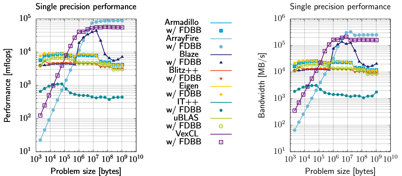
Figure 14: Compute performance (left) and memory bandwidth (right) for the expression given in Eq. (2) computed in single precision with the different linear algebra back-ends on CPUs and GPUs.
