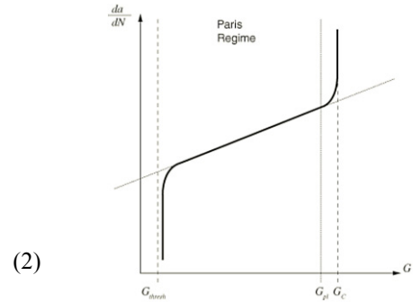
(2) Figure 2 Fatigue crack growth (Abaqus V. 6.14 Documentation, 2014)
