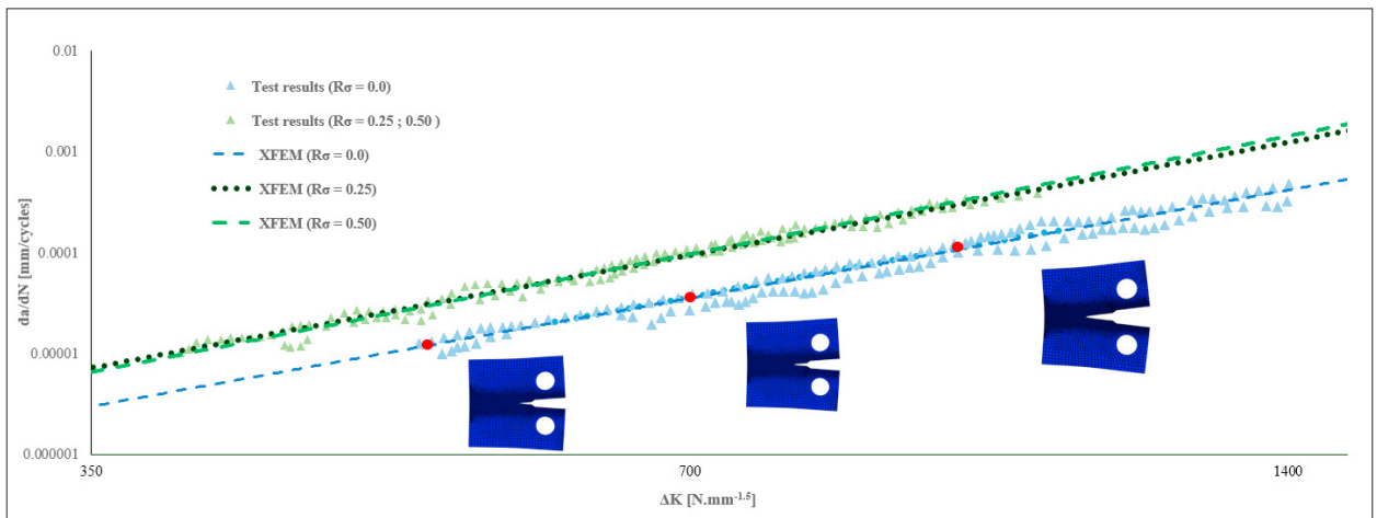
Figure 4 Fatigue crack propagation rates obtained from the numerical simulation compared with the test results
