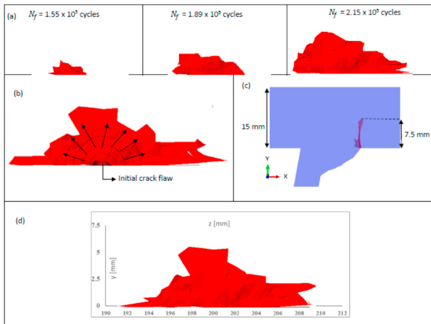
Figure 6 (a) Stages of crack propagation displayed as STATUSXFEM output (b) XFEM crack simulation including the initial semi-elliptical crack (c) Side view corresponding with the weld toe crack simulation (d) Crack front dimension
