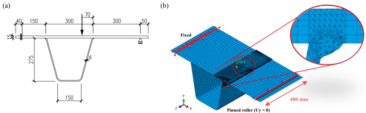
Figure 5 (a) Geometry of the OSD specimen (Nagy, 2016) (b) XFEM model: Boundary conditions and mesh quality
