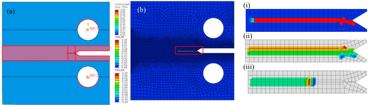
Figure 3 (a) XFEM model (b) Output results (i) STATUSXFEM (ii) PHILSM variable output (iii) PSILSM variable output
