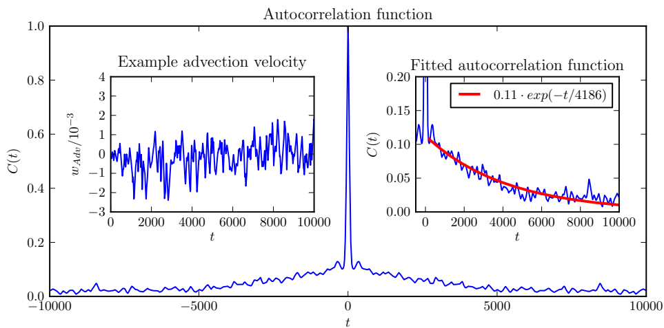
Figure 2. Statistics of transverse shift velocities determined by symmetry projection onto the span wise degrees of freedom. The inset shows that the velocities are small and fluctuate randomly. The correlation function (main frame) shows a strong central peak, indicative of weak correlations, and a broad tail reaching out to very long times. The right inset shows that this tail is well captured by an exponential distribution with a characteristic time of more than 4000 natural units.
